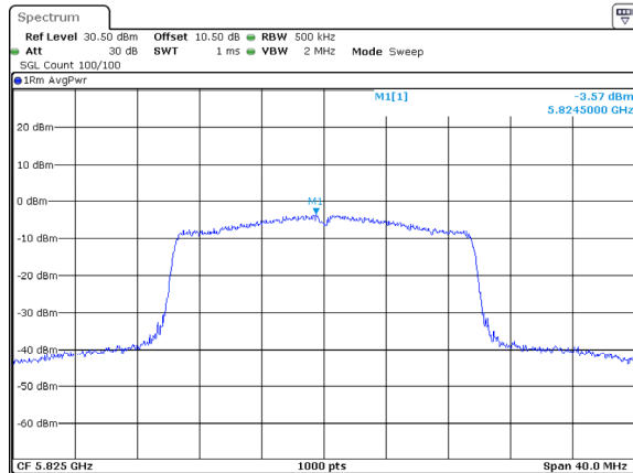
802.11ax20_5825MHz_RU_Full_Chain 1
