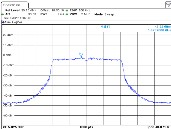
802.11a_5825MHz_Chain 1
