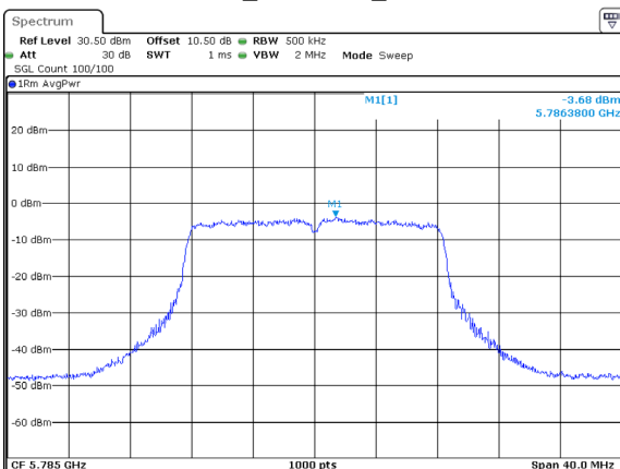
802.11a_5785MHz_Chain 2
