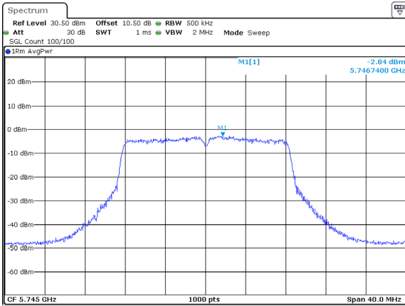
802.11a_5745MHz_Chain 1
