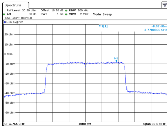
802.11ax40_5755MHz_RU_Full_Chain 1
