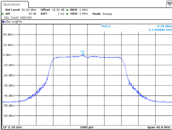
802.11a_5180MHz_Chain 1
