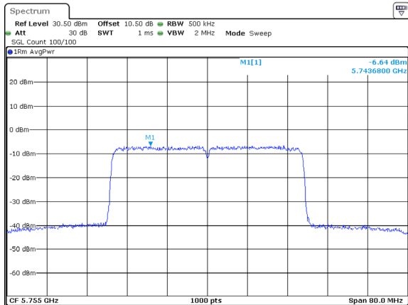
802.11ax40_5755MHz_RU_Full_Chain 2
