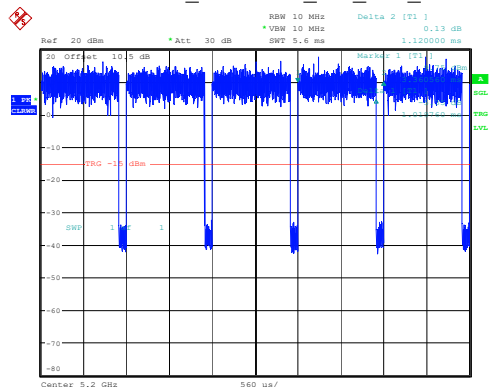
802.11ax20_5200MHz_RU_Full_Chain 1
