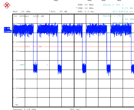
802.11ax40_5190MHz_RU_Full_Chain 1
