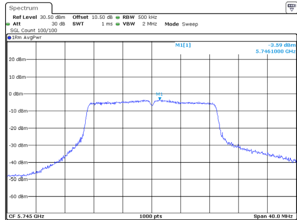
802.11ac20_5745MHz_Chain 2
