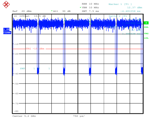
802.11a_5200MHz_Chain 1
