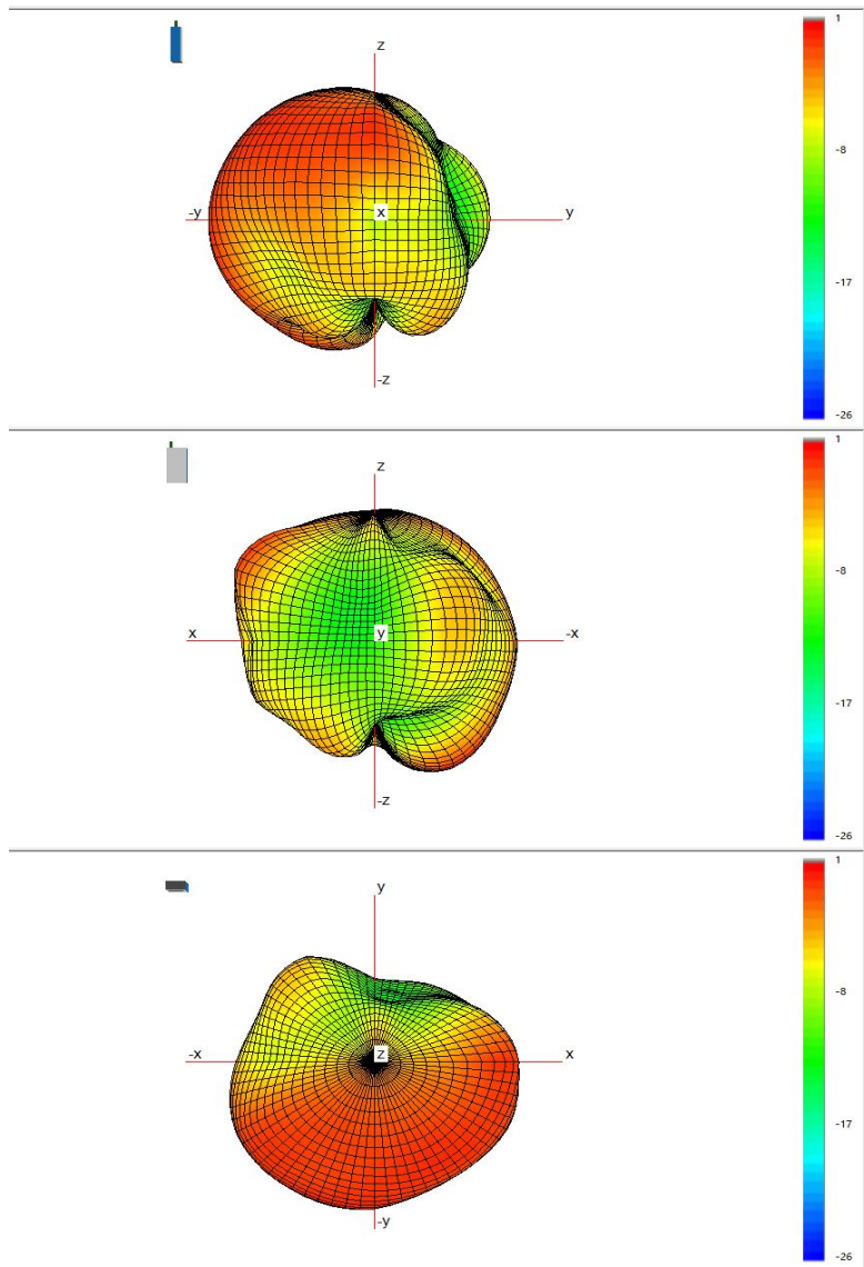
2D sky map (X->Y;X->Z;Y->Z)
