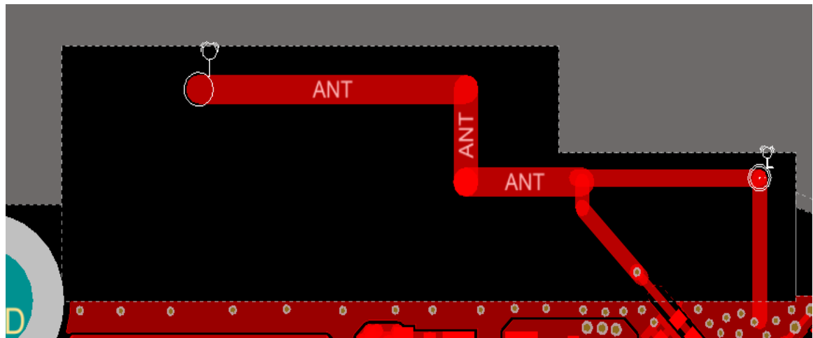
Antenna Photo
