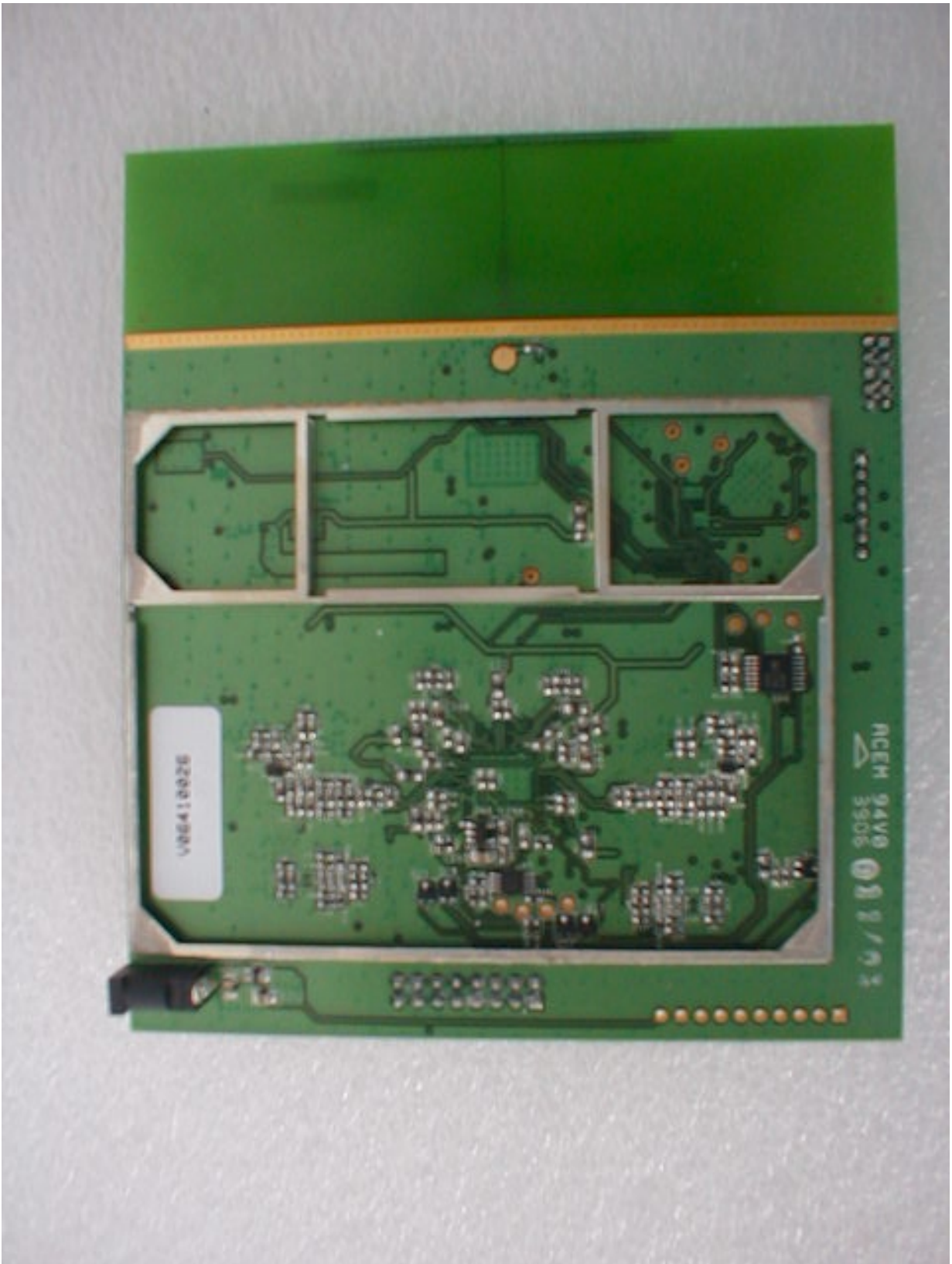
BOTTOM VIEW OF MAIN BOARD (CIRCUIT SHIELDS REMOVED)
