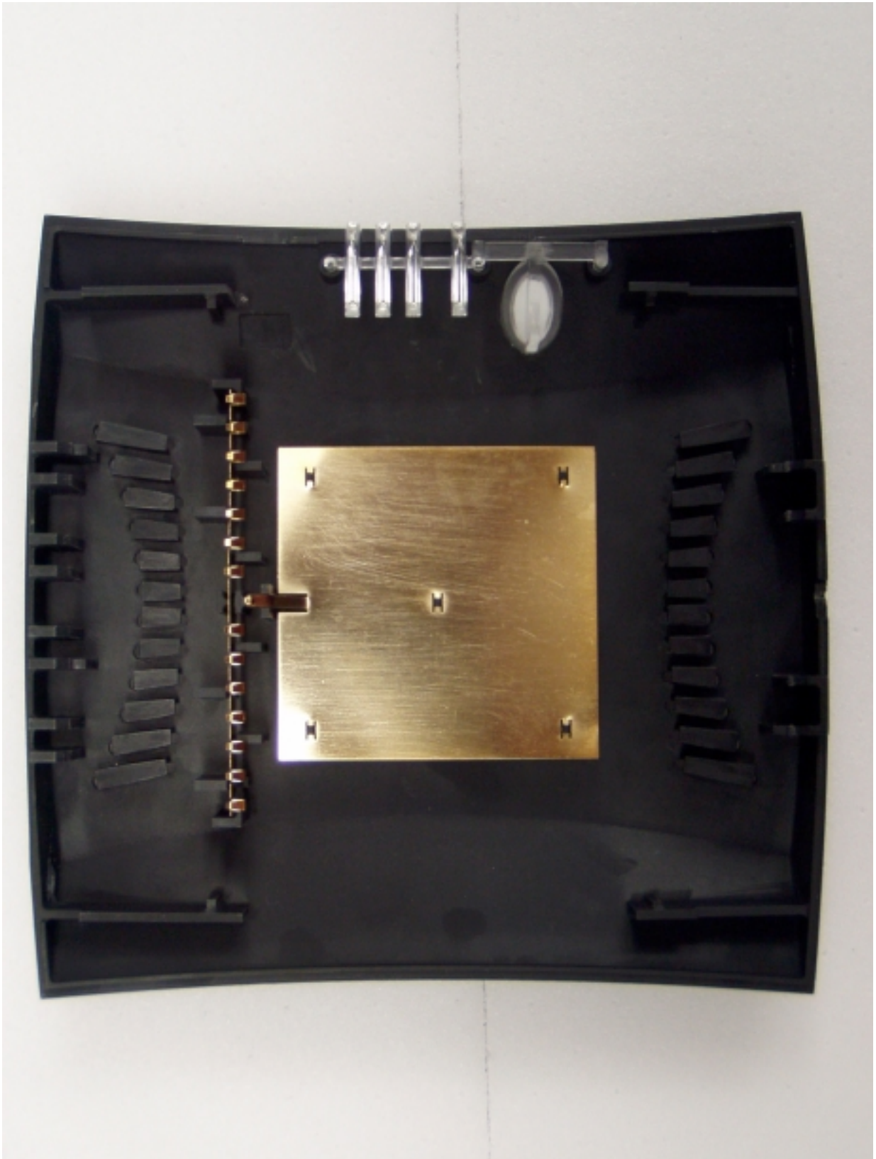
VIEW OF PATCH ANTENNA, MOUNTED INSIDE CHASSIS
