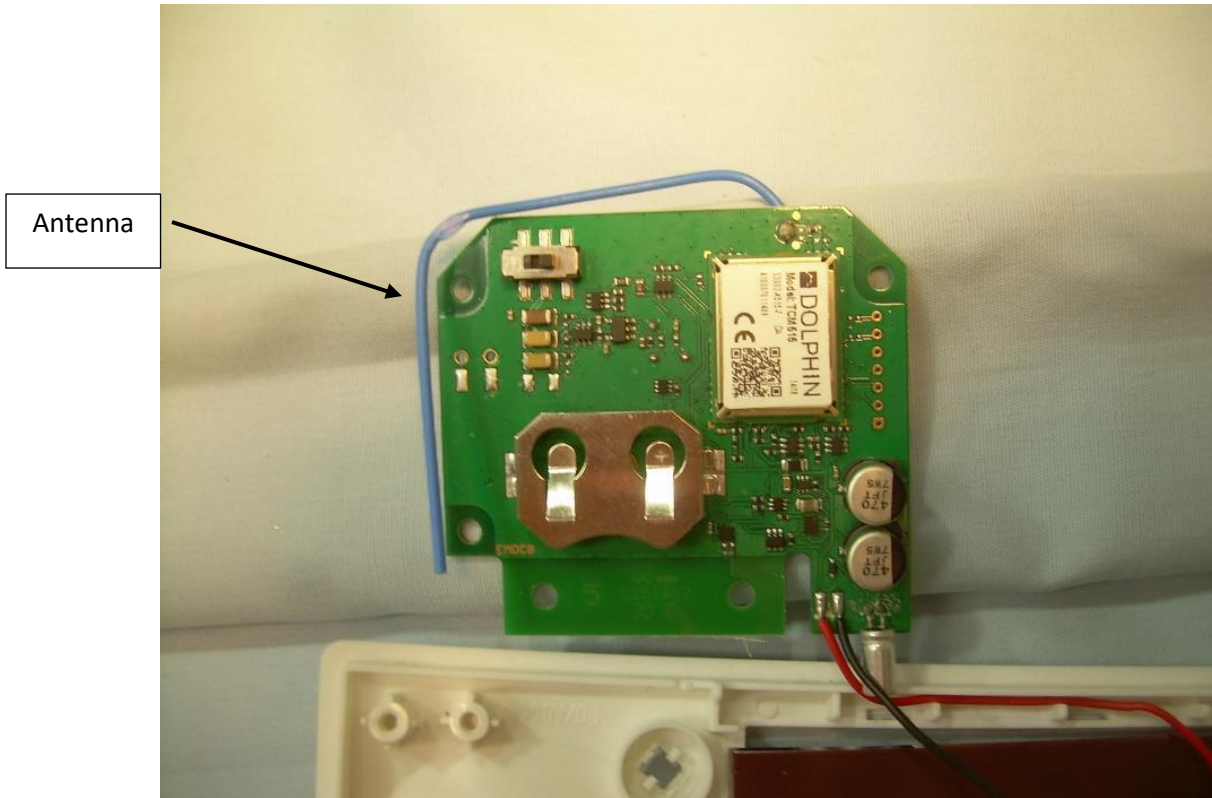
Photograph 2 – Bottom View of the PCB
