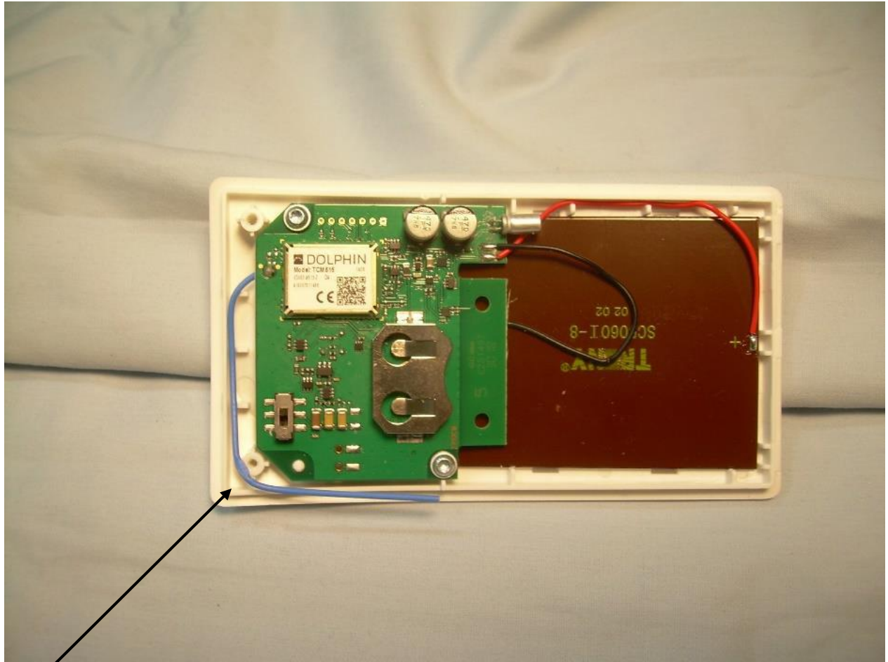
Photograph 3 – View of PCBA Mounting in Housing
