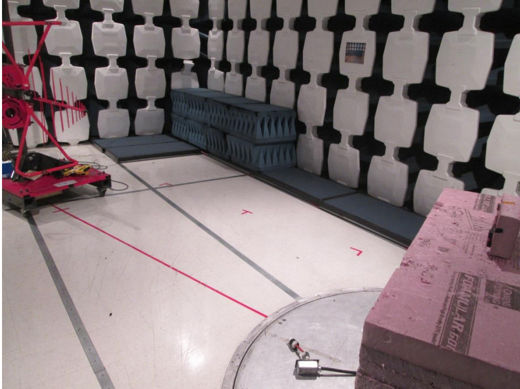
Radiated Emissions, 30-1000MHz, Rear View, External Antenna EUT
