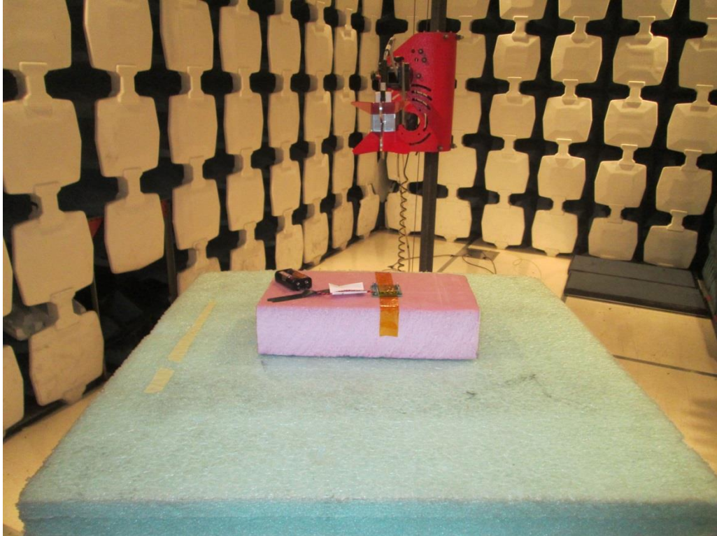
Radiated Emissions 6-18GHz, Rear View
