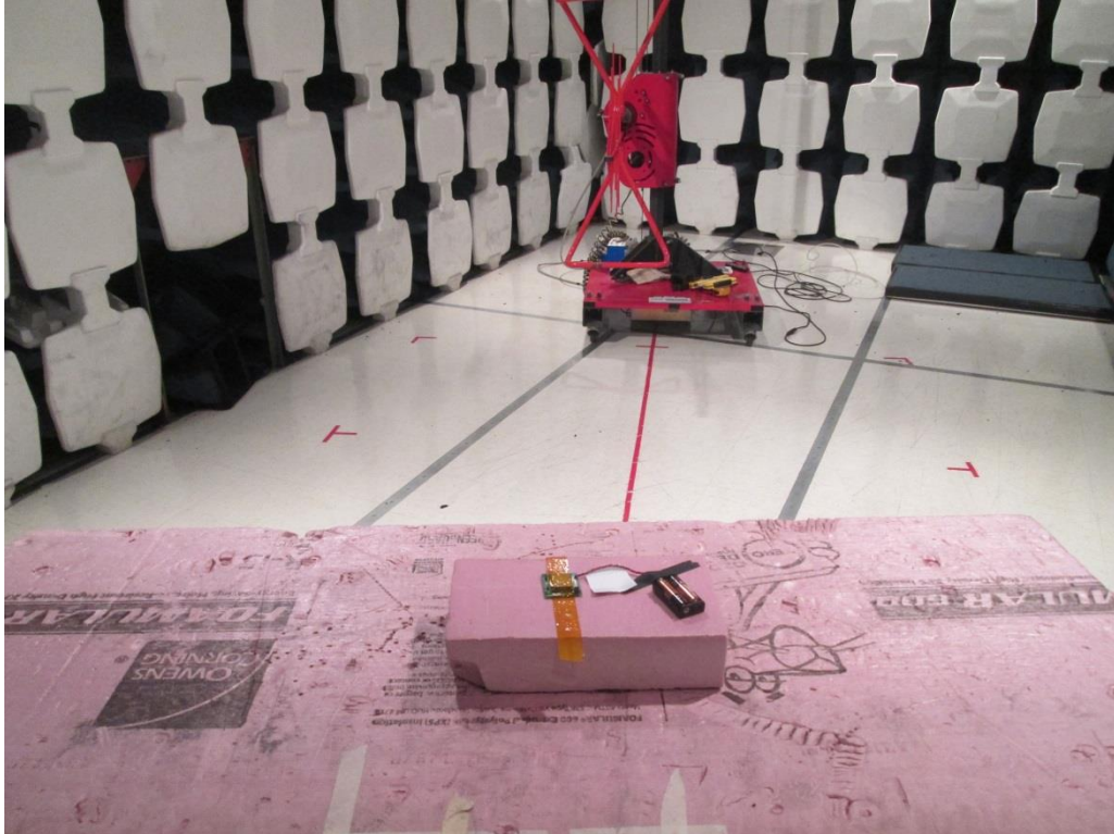
Radiated Emissions, 30-1000MHz, Rear View, Trace Antenna EUT
