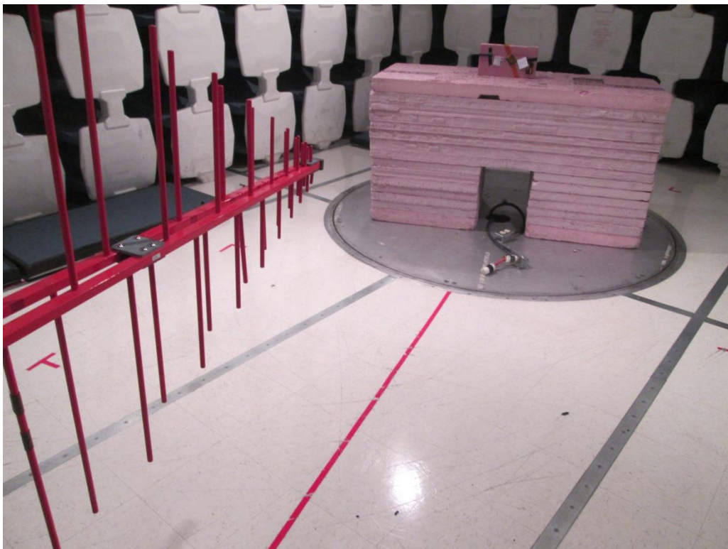
Radiated Emissions, 30-1000MHz, Front View, External Antenna EUT
