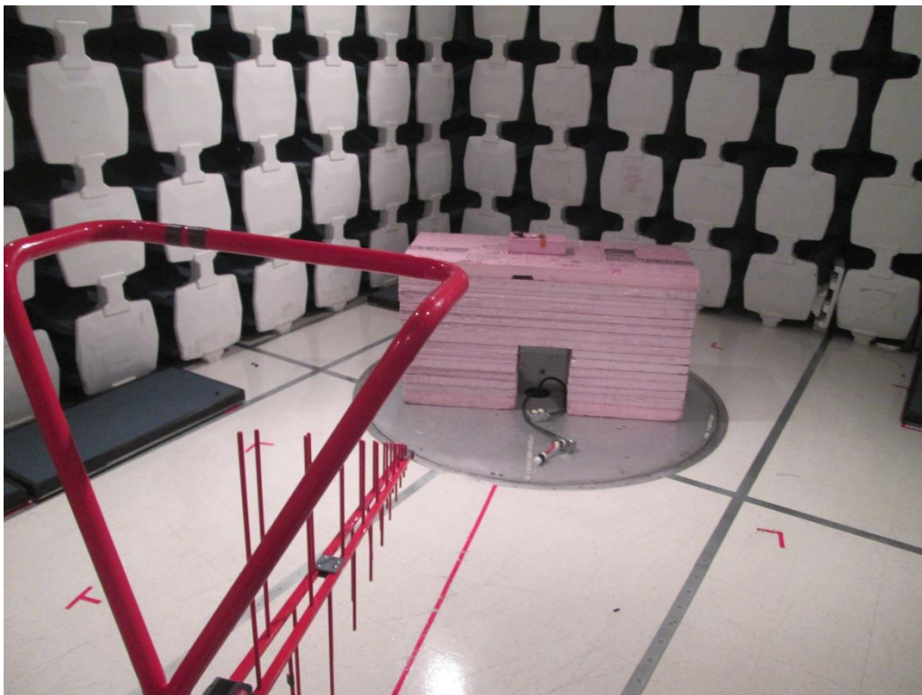
Radiated Emissions, 30-1000MHz, Front View, Trace Antenna EUT
