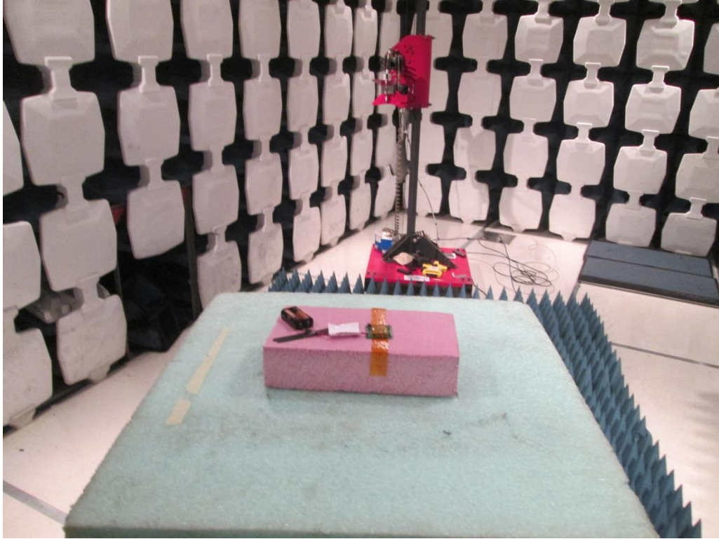
Radiated Emissions 1-6GHz Rear View
