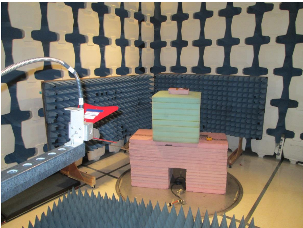
Radiated Emissions 1-6GHz, Front View
