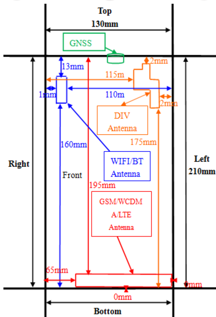
Antenna Configuration 1- LT800H
