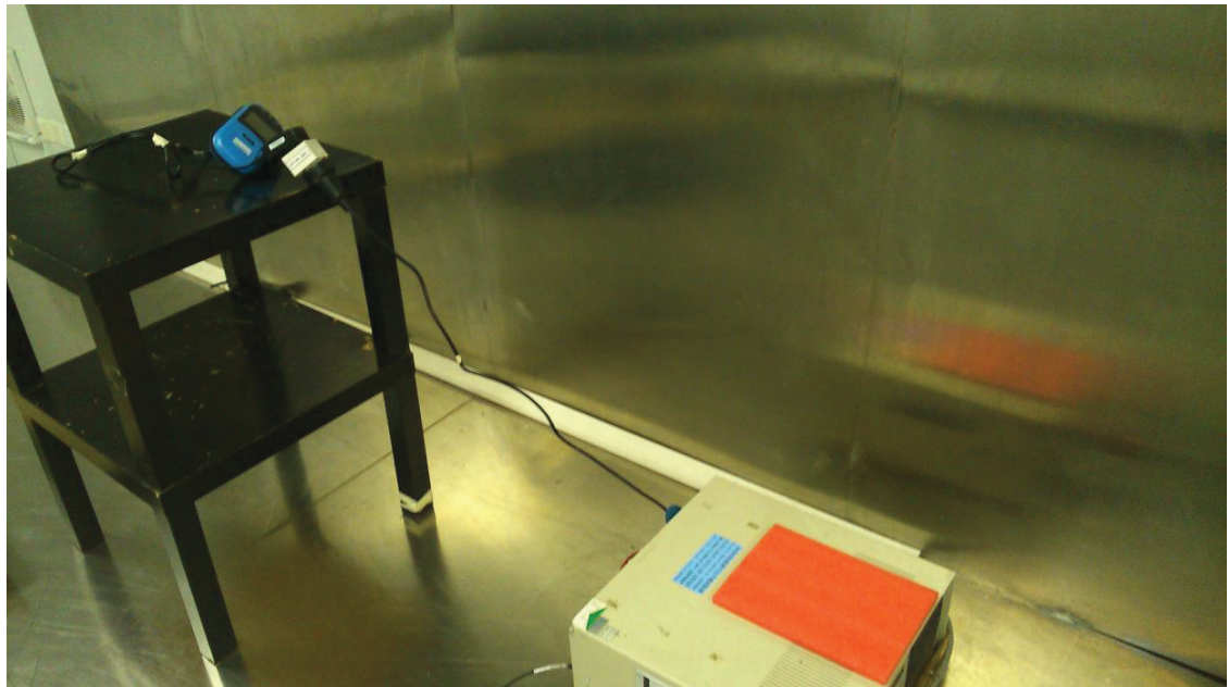
Conducted Emissions
