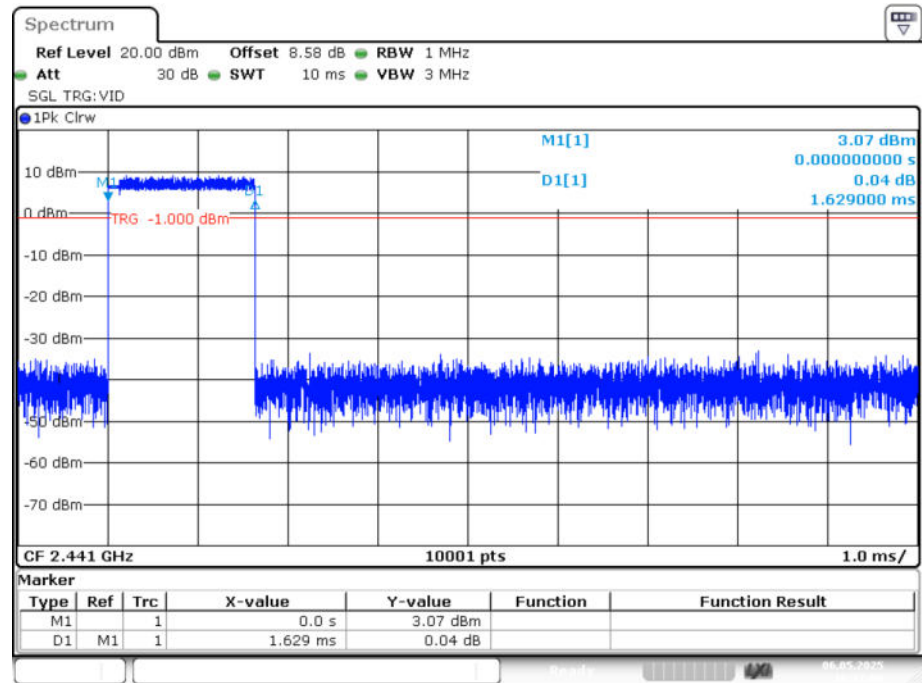
Dwell NVNT 3-DH3 2441MHz Ant1 One Burst
