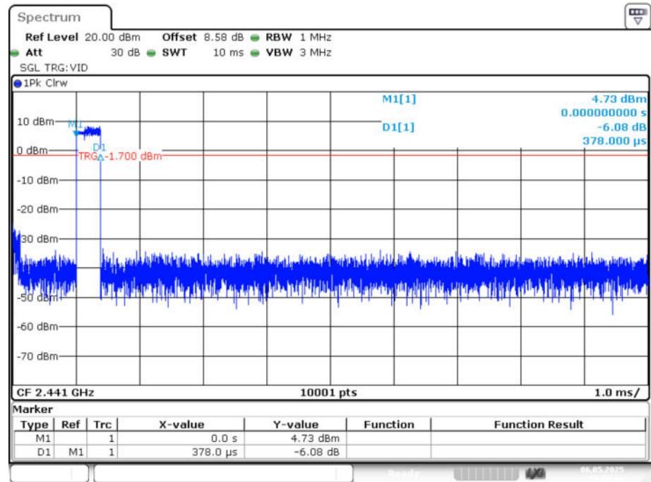
Dwell NVNT 2-DH1 2441MHz Ant1 One Burst
