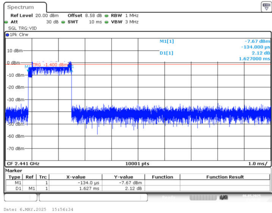
Dwell NVNT 2-DH3 2441MHz Ant1 Accumulated
