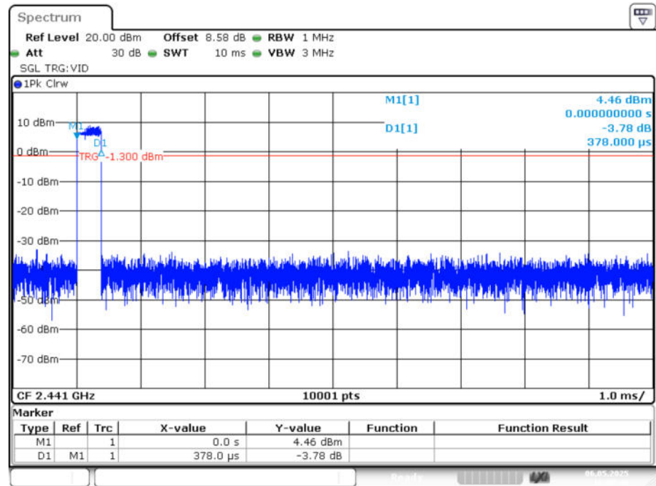
Dwell NVNT 3-DH1 2441MHz Ant1 One Burst
