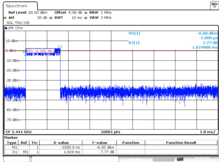
Dwell NVNT 1-DH3 2441MHz Ant1 One Burst
