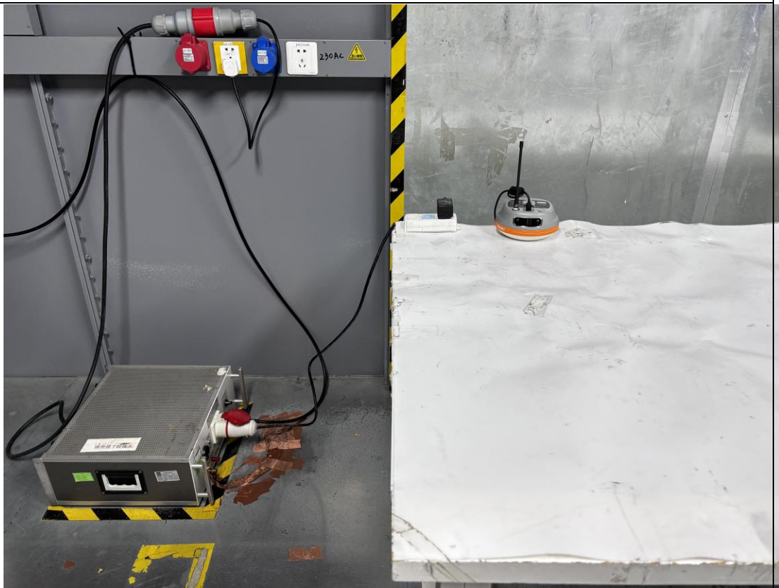
Conducted emission
