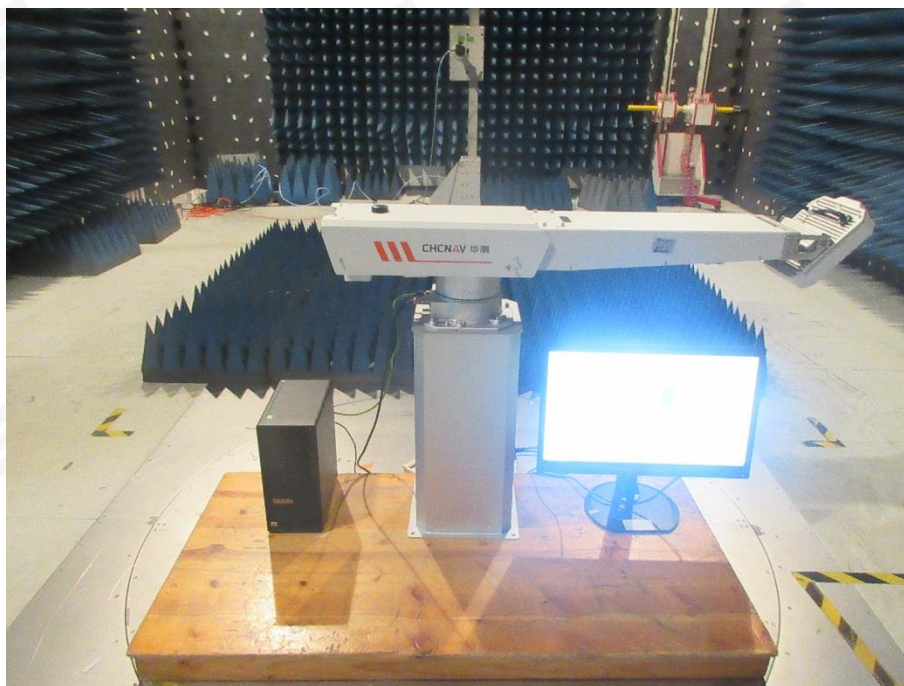
18G-40G radiation
