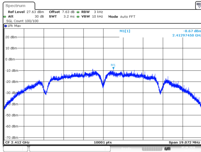
PSD NVNT 802.11b 2412MHz Ant1
