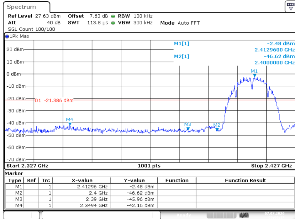
Band Edge NVNT 802.11b 2412MHz Ant1 Emission
