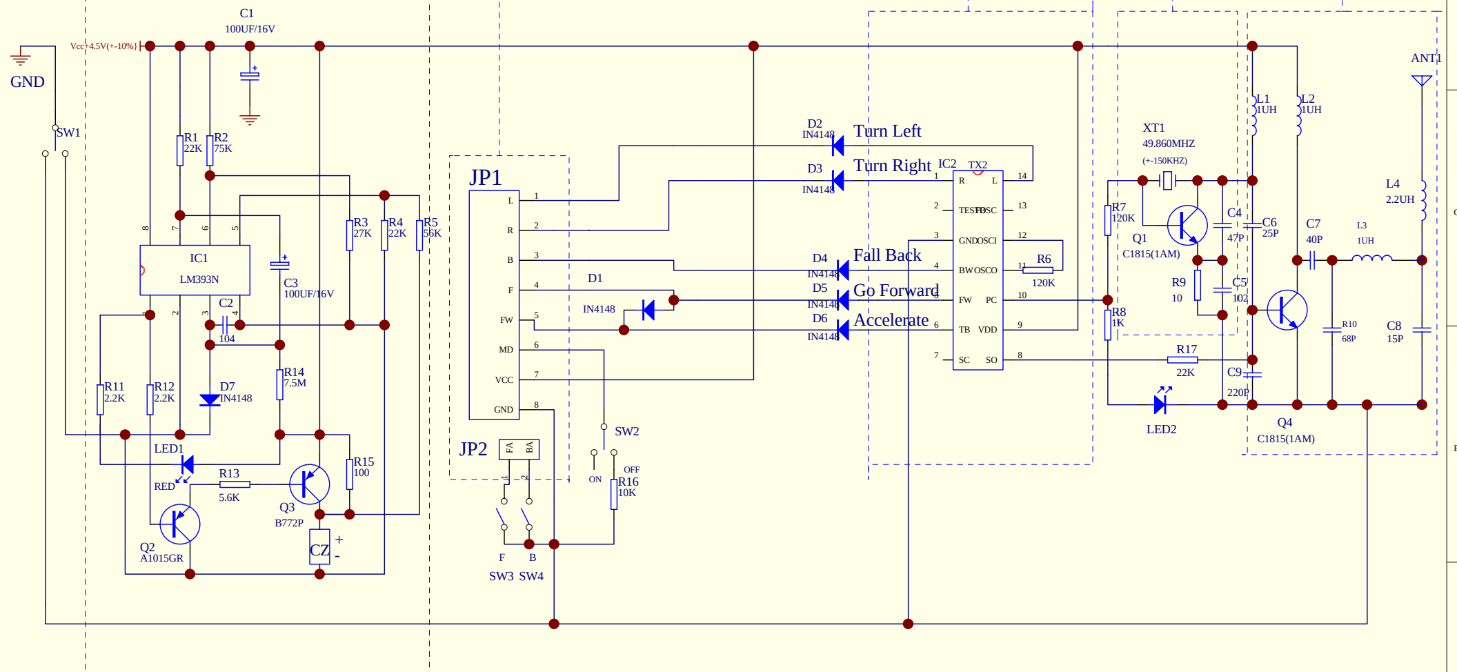
TRANSMITTER CIRCUIT DIAGRAM---T0402-1
