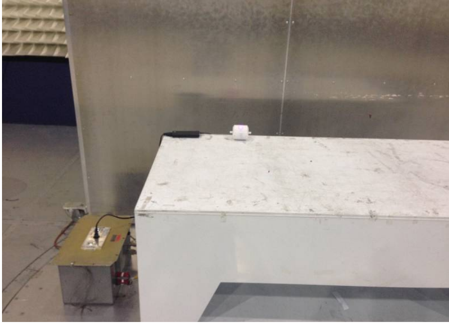
AC Line Conducted Emissions
