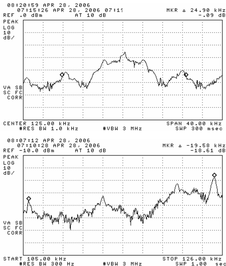
Figure 6.3. Measured worst case bandwidth of the DUT. (maximum modulation rate)
