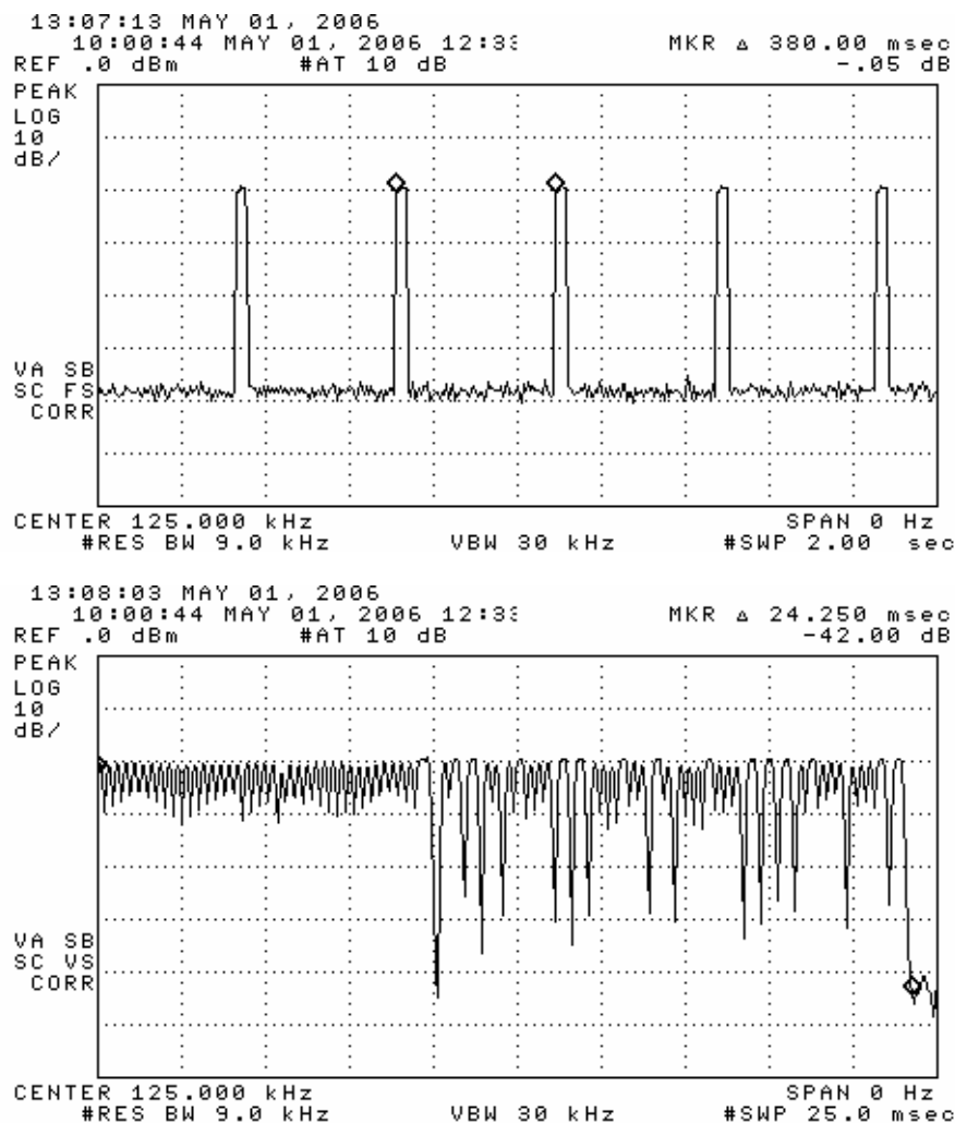
Figure 6.1(b). Transmission modulation characteristics. High Data-rate Mode
