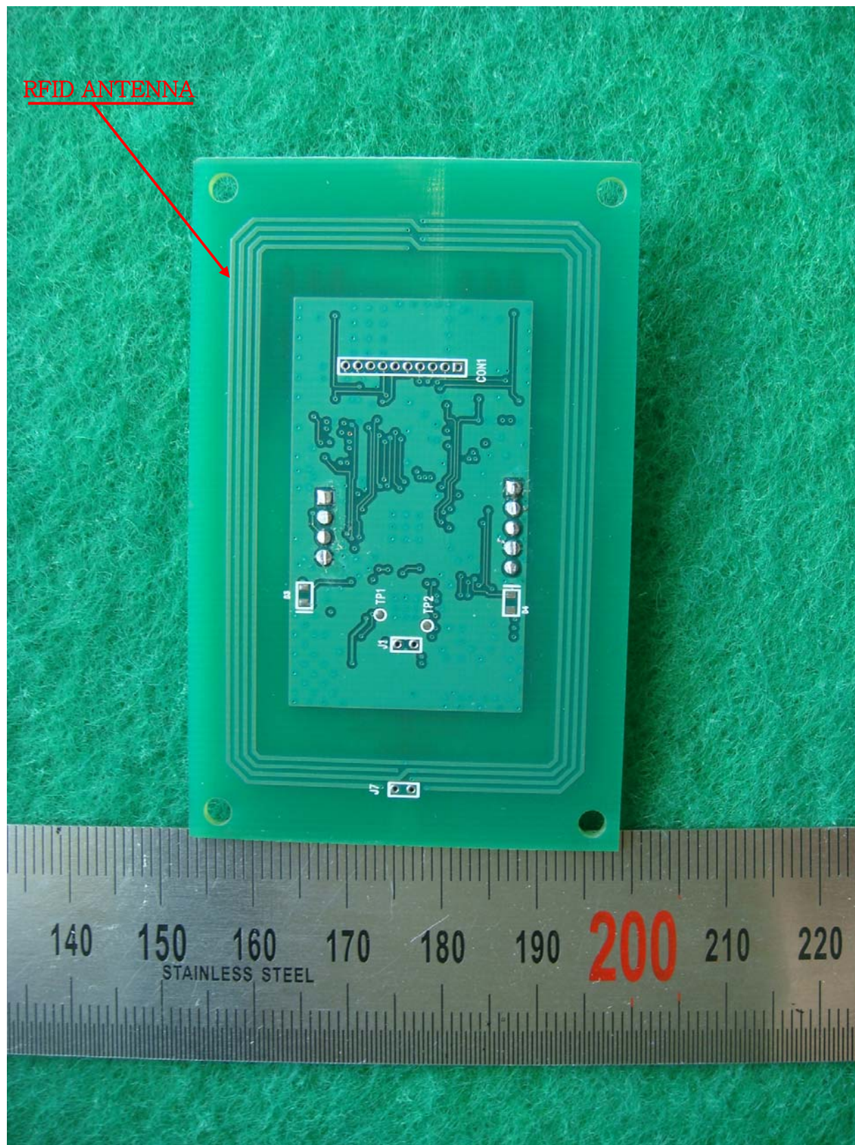
<Photograph 2: RF board - Rear view>
