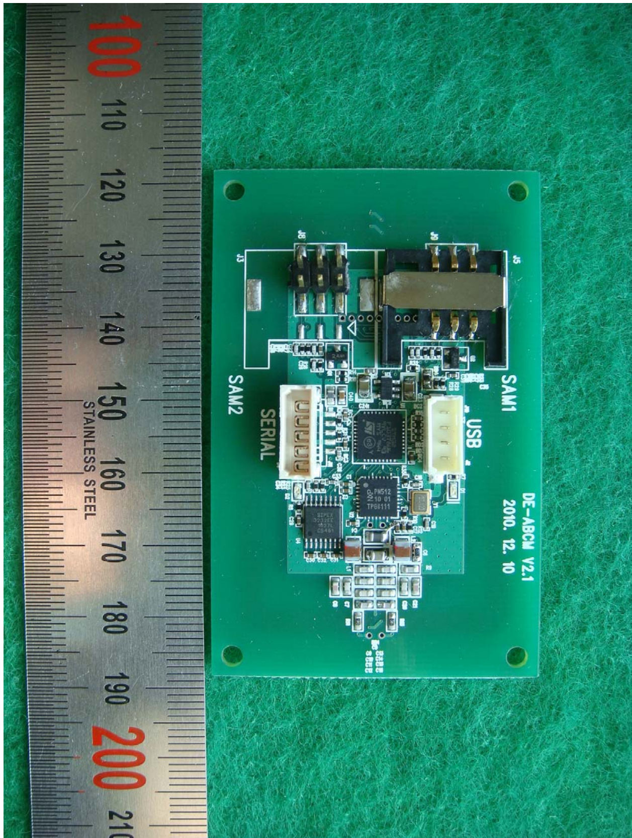
<Photograph 1: RF board - Front view>
