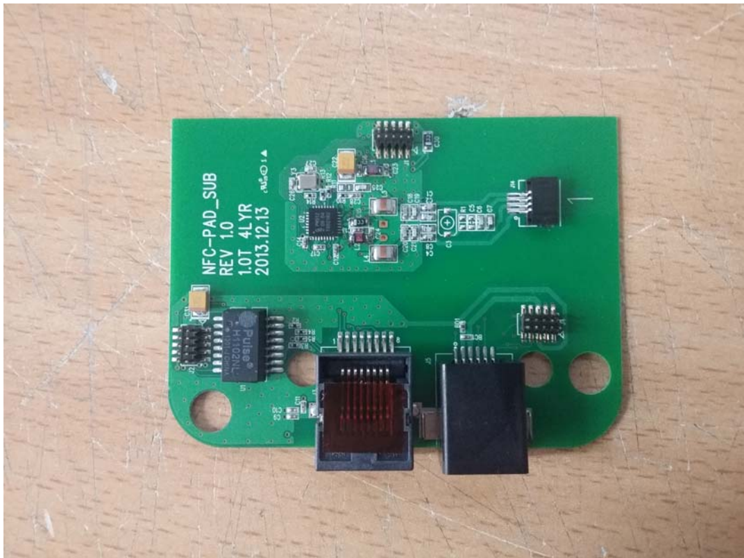
Sub board
