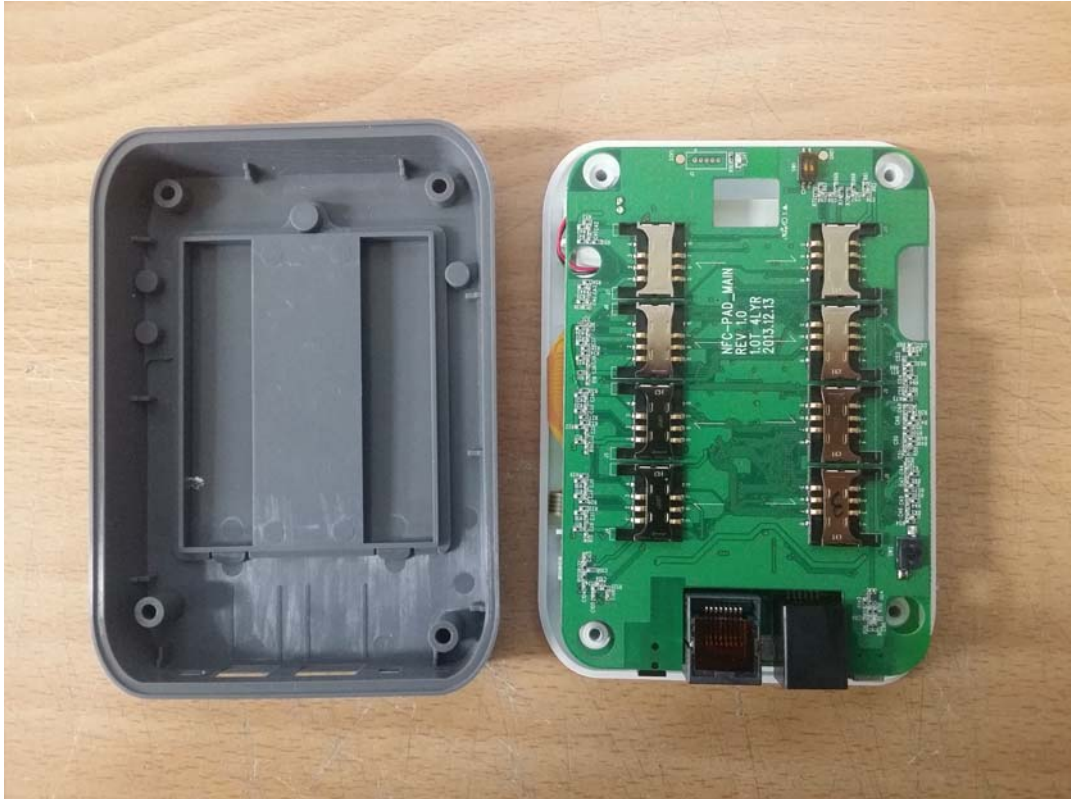
Cover opened
