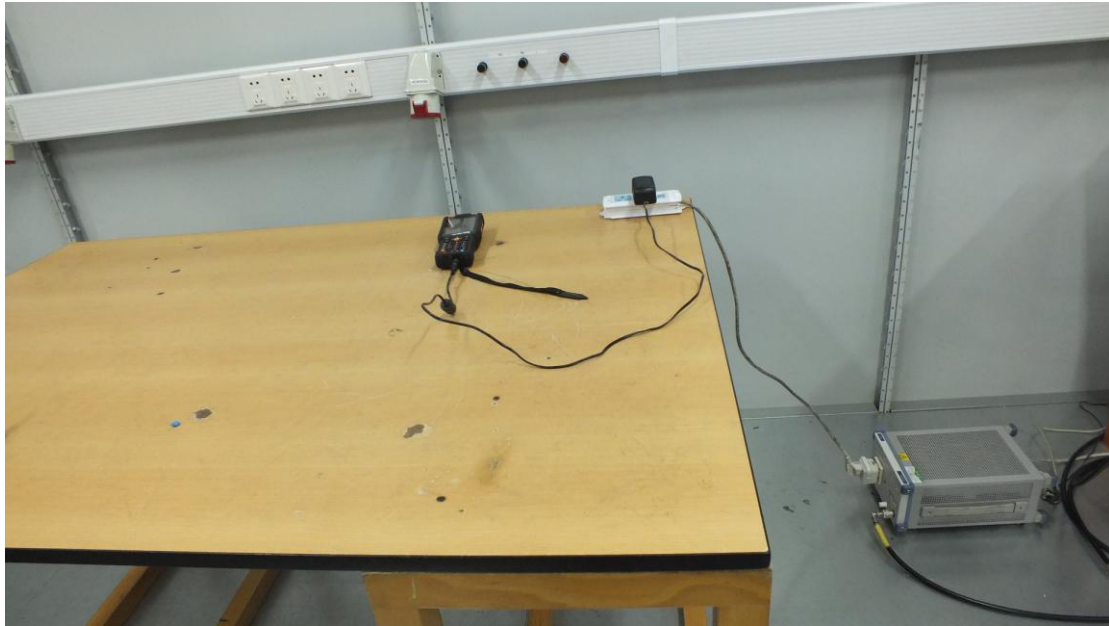
AC Conducted Emission Test Setup
