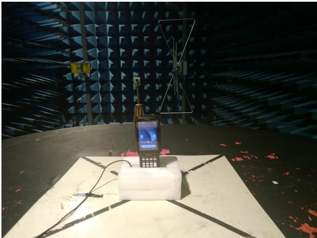
FCC Part15C Radiated Emission above 18-25GHz -Front
