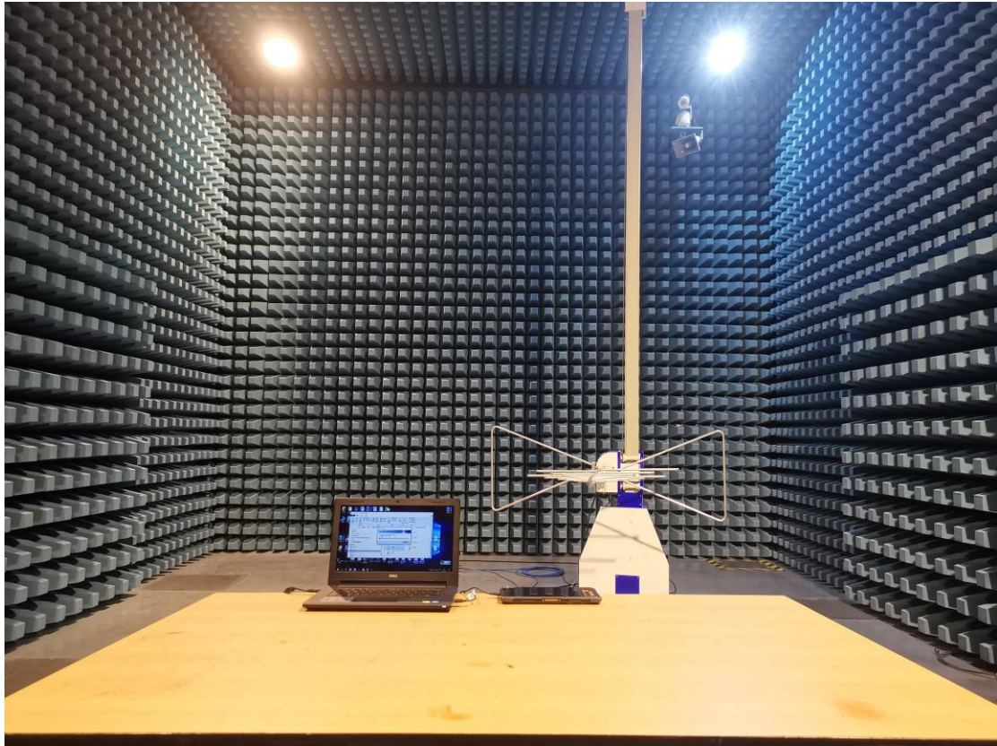
FCC Part15B Radiated Emission below 1GHz -Front
