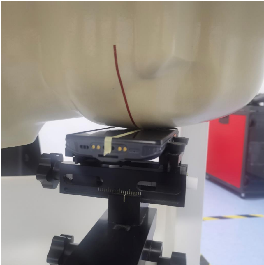
Left Head Cheek
