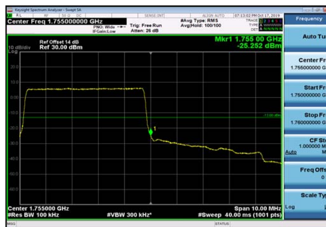
HighRange_FDD04_10MHz_1750_OneRB _high_QPSK
