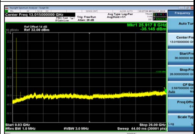
FDD12_LowRange_1.4MHz_30MHz~26GHz
