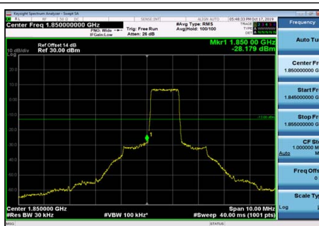
LowRange_FDD02_1.4MHz_1850.7_fullRB _Low_QPSK
