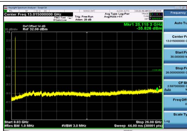
FDD12_HighRange_5MHz_30MHz~26GHz
