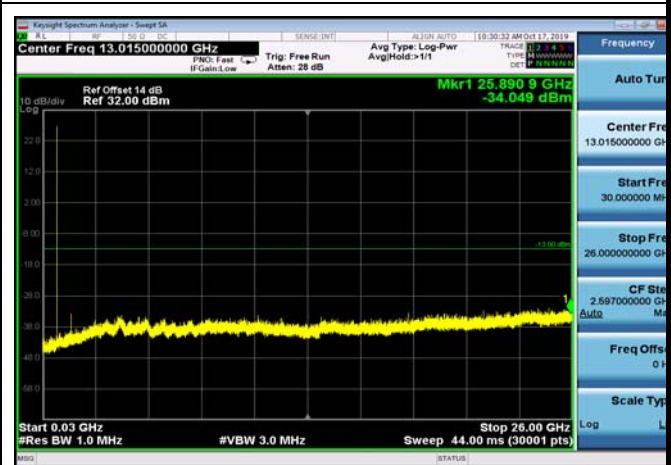
FDD12_HighRange_3MHz_30MHz~26GHz
