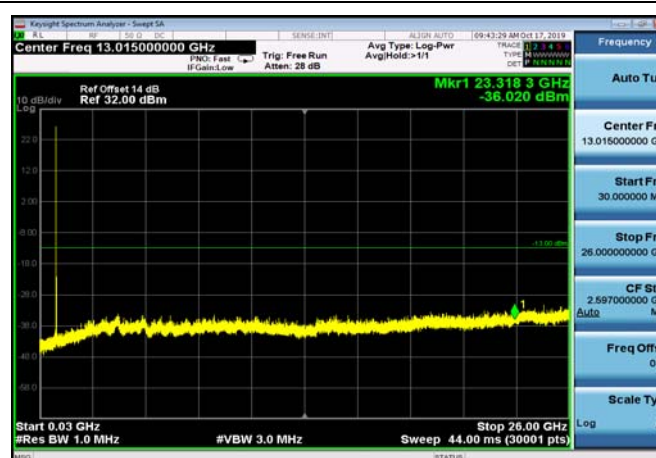
FDD05_MidRange_10MHz_30MHz~26GHz
