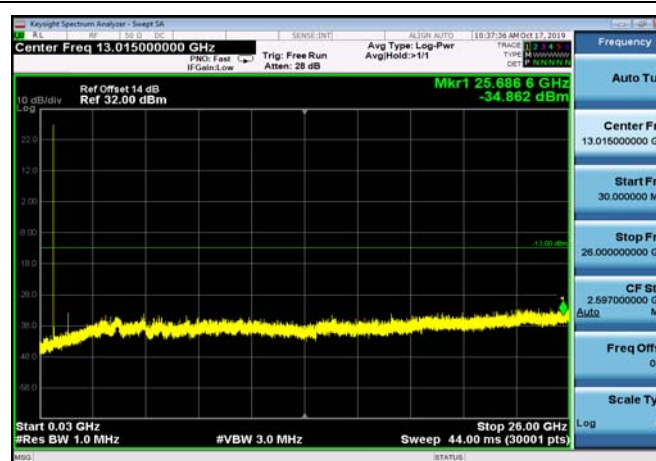
FDD17_LowRange_5MHz_30MHz~26GHz
