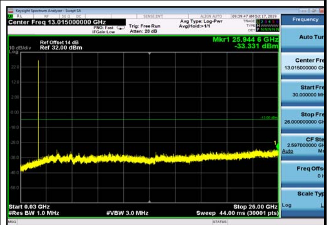
FDD02_LowRange_3MHz_30MHz~26GHz
