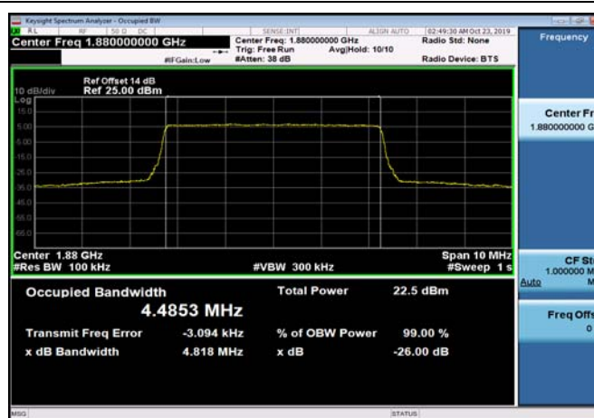
FDD02_MidRange_5_1880_QPSK
