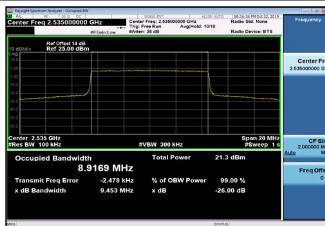
FDD07_MidRange_10MHz_2535MHz_Q16
