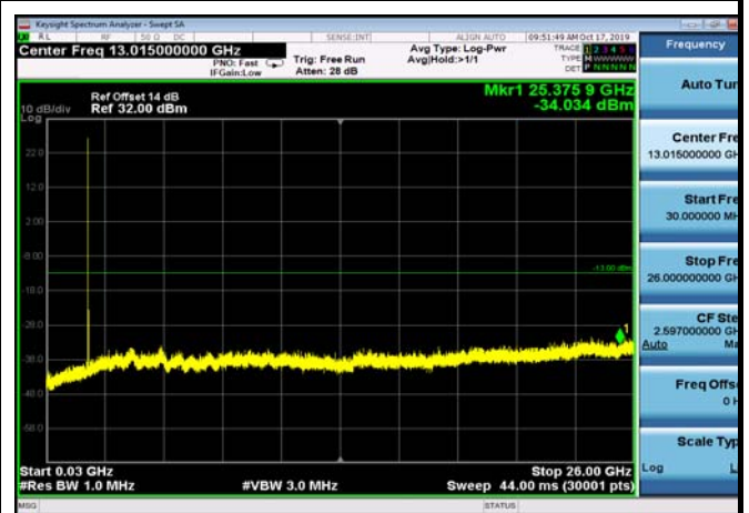
FDD02_MidRange_3MHz_30MHz~26GHz
