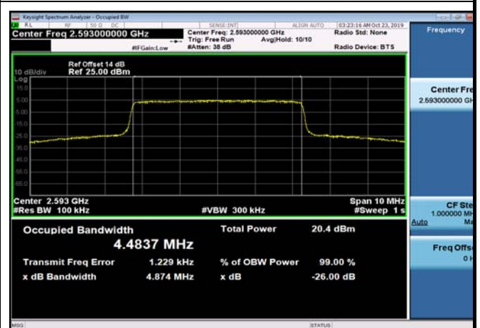
TDD41_MidRange_5_2593_Q16
