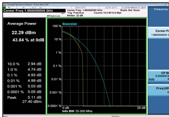
FDD02_LowRange_20MHz_1860_OneRB _high_Q16
