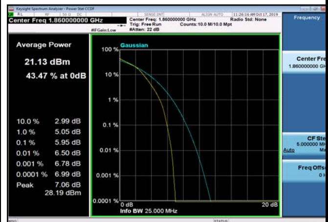
FDD02_LowRange_20MHz_1860_fullRB _Q16
