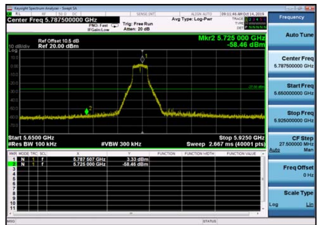
U-NII-3 ,Plot 1,Band Edge-802.11a(20M Hz),5785MHz,Ant2
