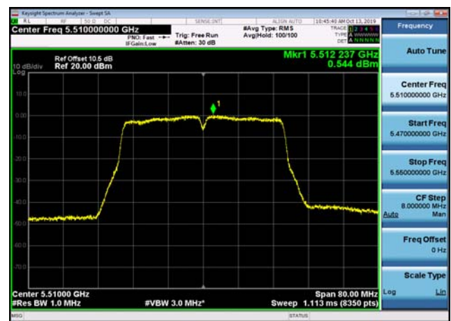
U-NII-2c Power spectral density-802.1 1n(40MHz),5510MHz,Ant2
