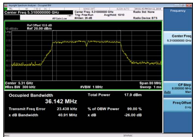
U-NII-2a 26dB Bandwidth-802.11n(40MHz ,5310MHz,Ant2
