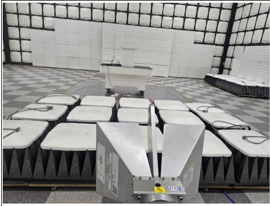
Photo of Radiated Spurious Emission Test (Above 18 GHz)
