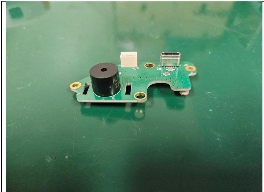
<Sub PCB Side View>
