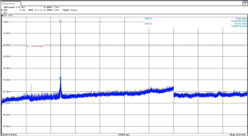
Conducted Spurious emission 9 kHz ~ 10 GHz - 2 402 Mhz (1M PHY)
