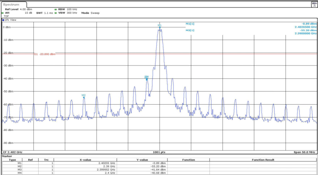
Conducted band edge plot - 2 402 Mhz (1M PHY)
