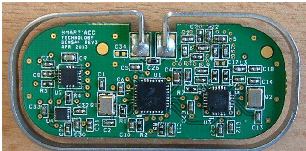
PCB view, with integral antenna
