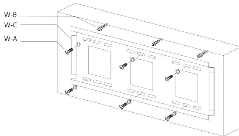
Figure 3-5 Install wallboard
