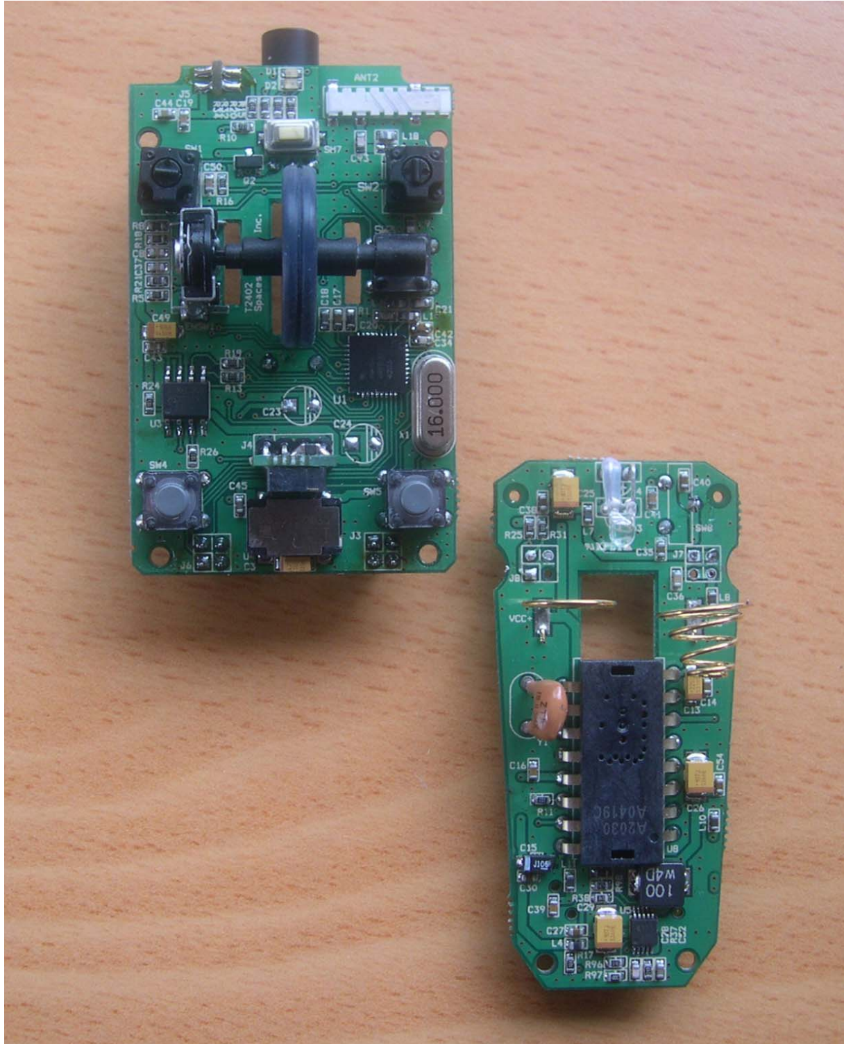
<Photograph 2: Front View - Main board>
