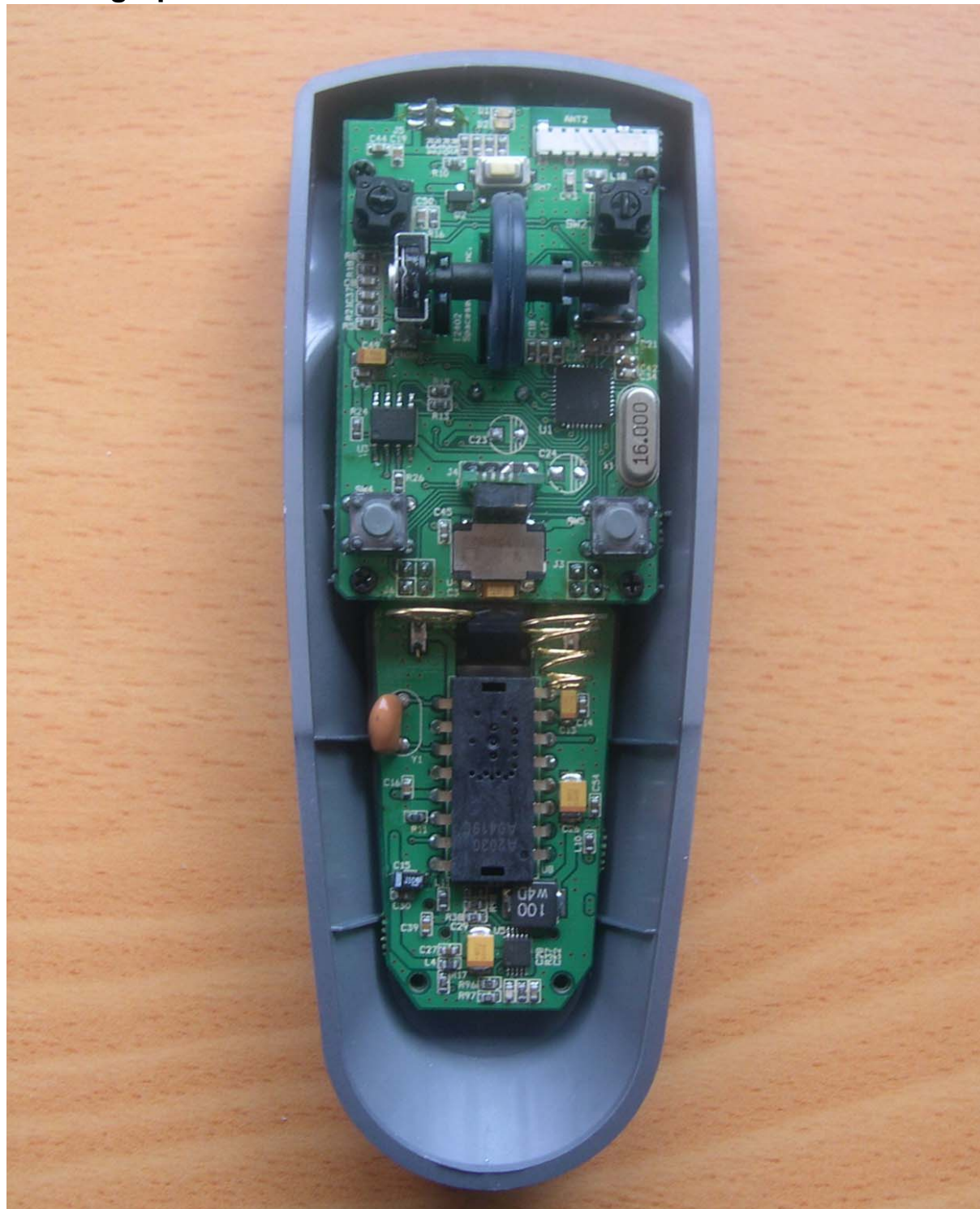
<Photograph 1: Cover removed>
