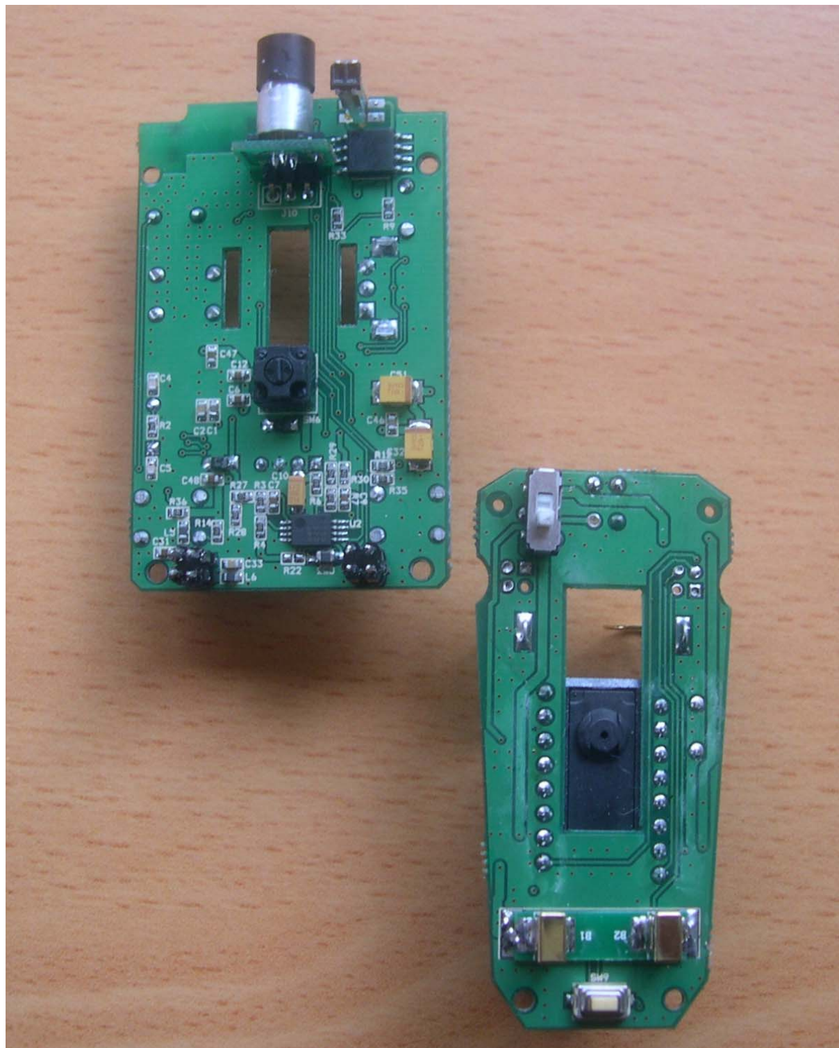
<Photograph 3: Rear View >
