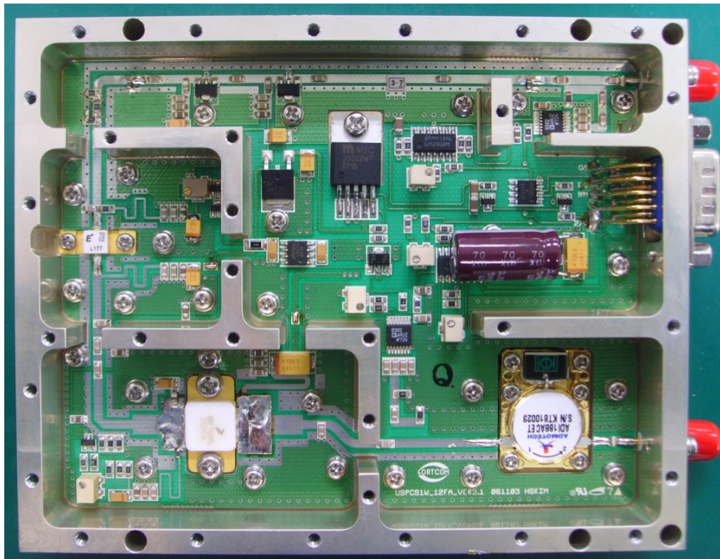
<Inner View>
