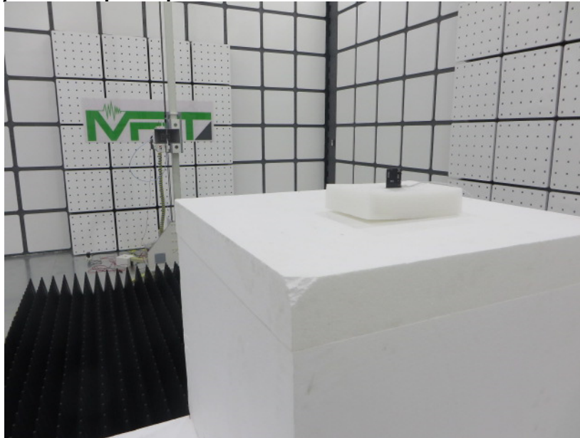
Photograph 3: Set-up for Spurious Emissions above 1GHz
