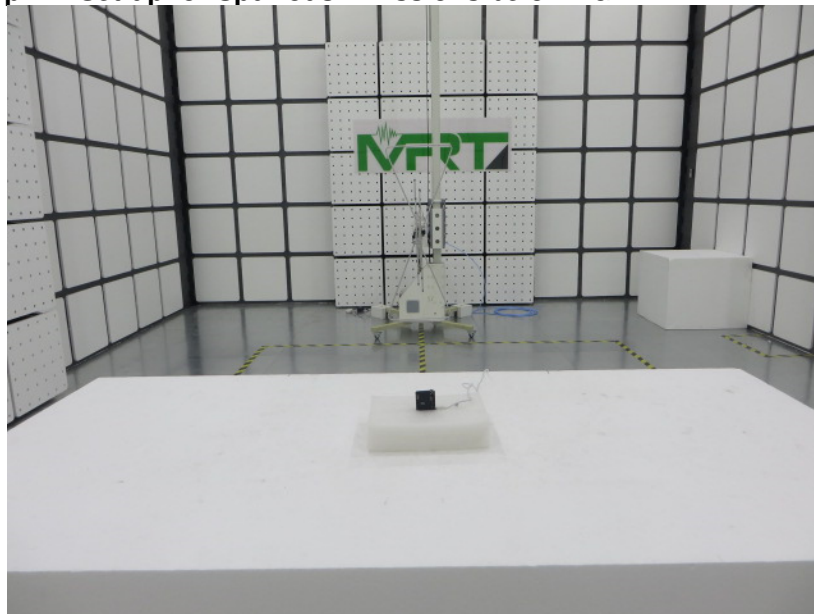
Photograph 2: Set-up for Spurious Emissions below 1GHz
