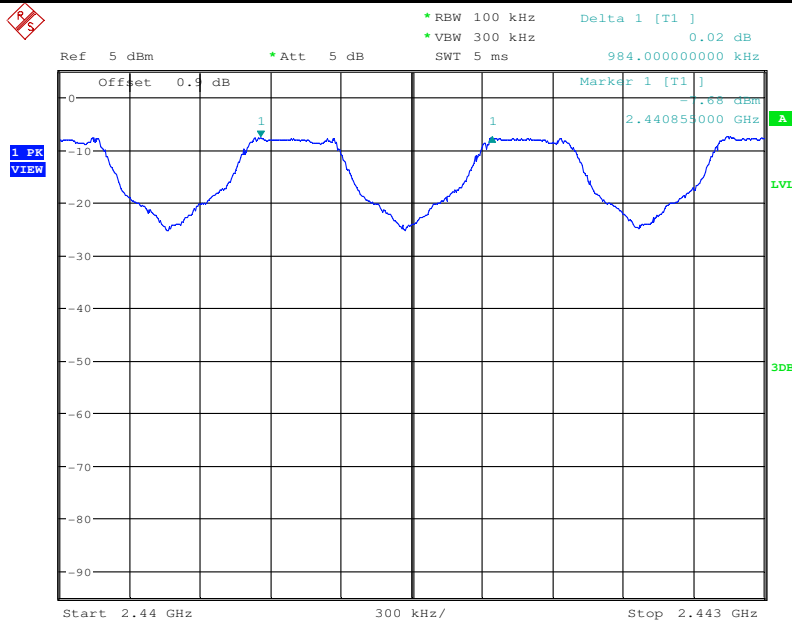
Carrier Frequency Separation_DH5_2441
