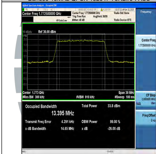
Band66-15MHz-QPSK-132597-75RB#0-PASS
