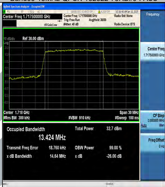
Band66-15MHz-16QAM-132047-75RB#0-PASS
