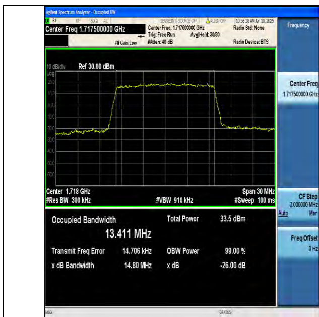
Band66-15MHz-QPSK-132047-75RB#0-PASS
