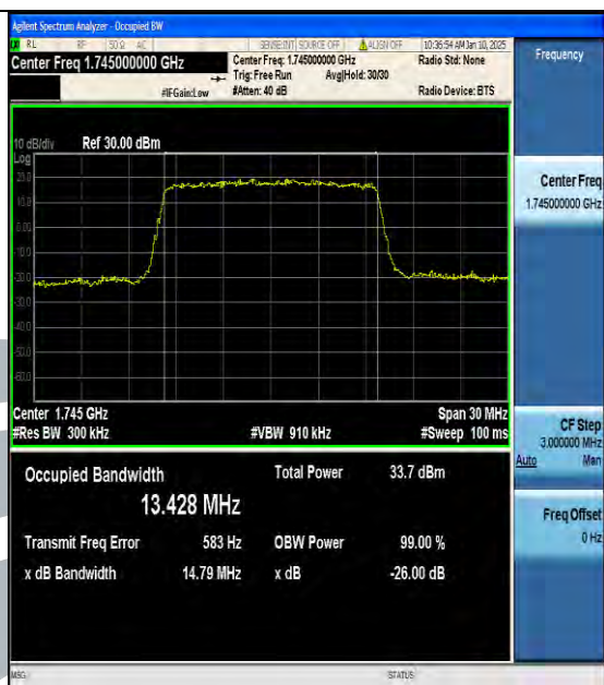
Band66-15MHz-QPSK-132322-75RB#0-PASS
