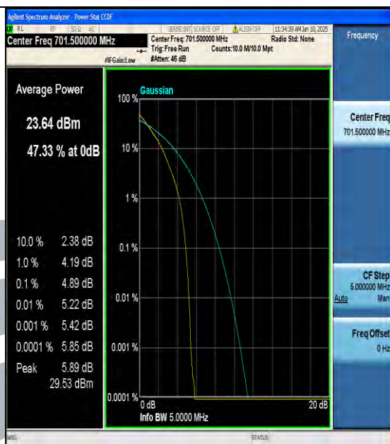
Band12-5MHz-QPSK-23035-25RB#0-PASS
