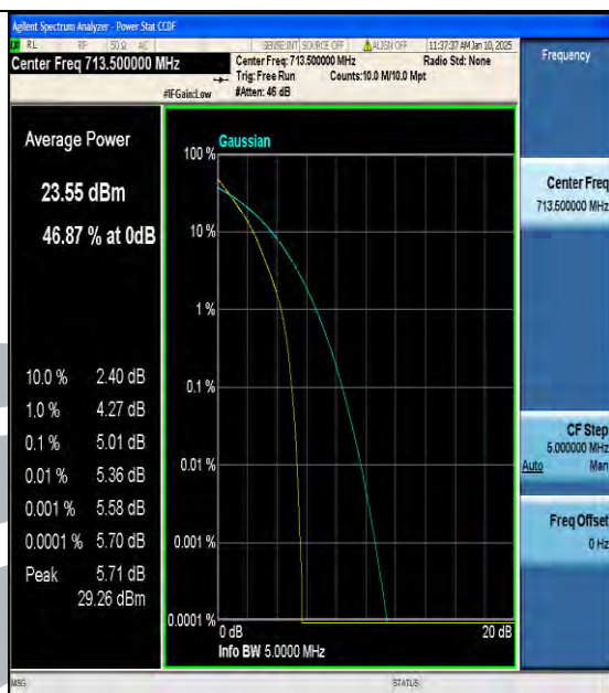
Band12-5MHz-QPSK-23155-25RB#0-PASS
