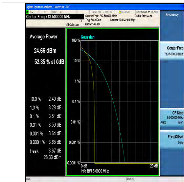
Band12-5MHz-QPSK-23155-1RB#0-PASS
