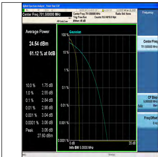
Band12-5MHz-QPSK-23035-1RB#0-PASS
