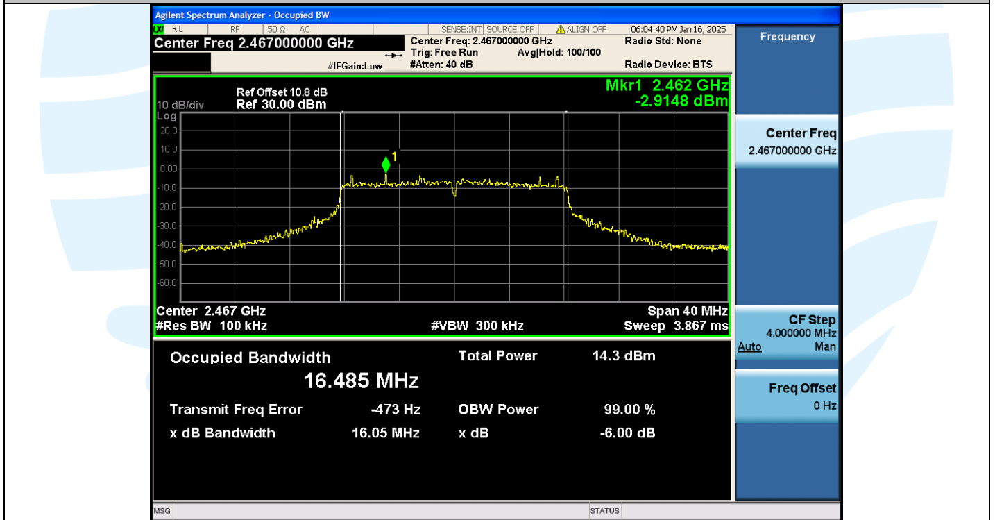
11G-Ant1-2467MHz-PASS
