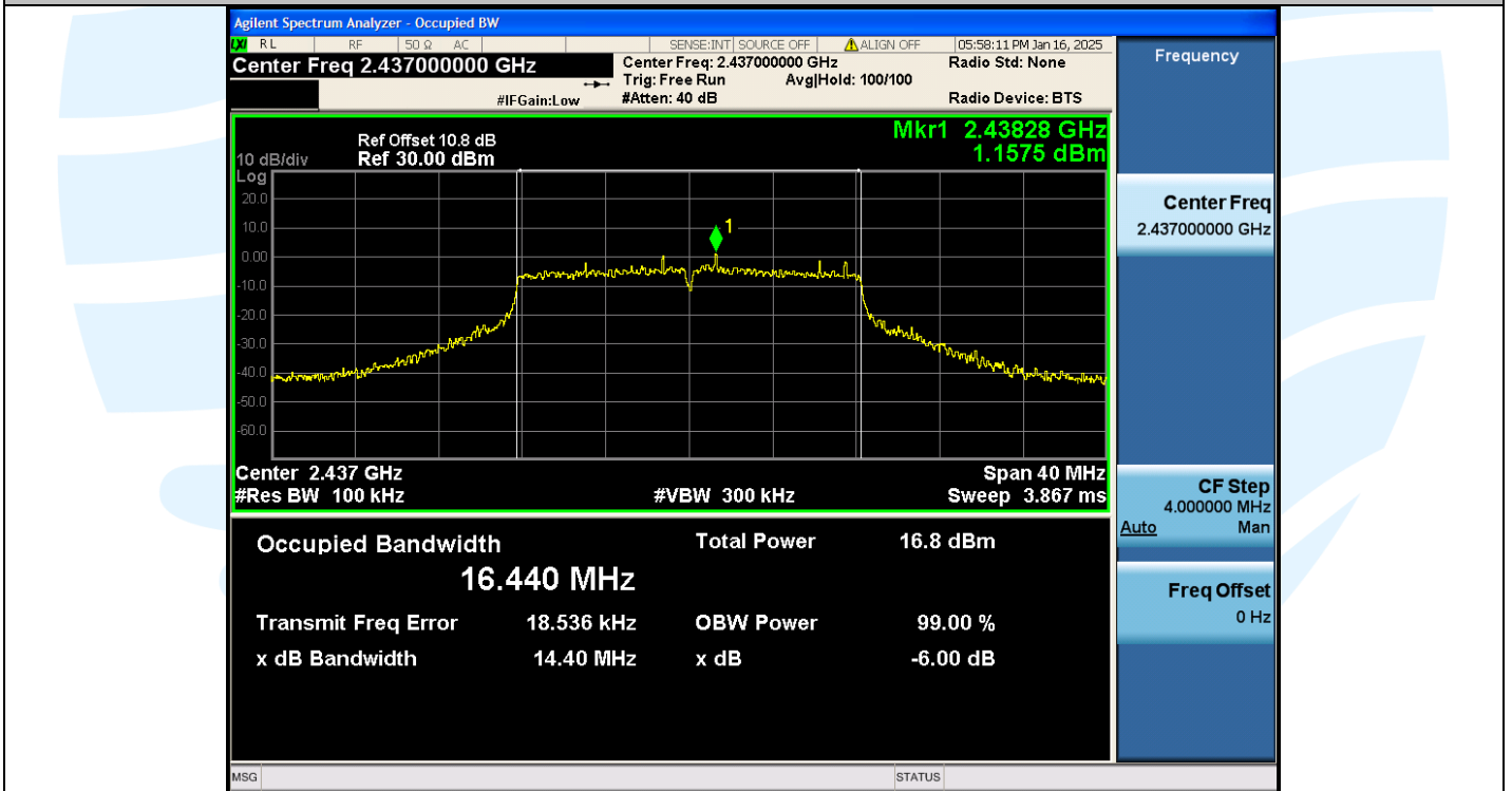
11G-Ant1-2437MHz-PASS
