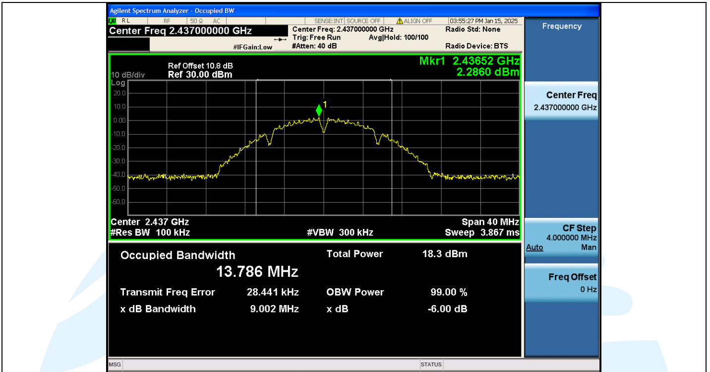
11B-Ant1-2437MHz-PASS
