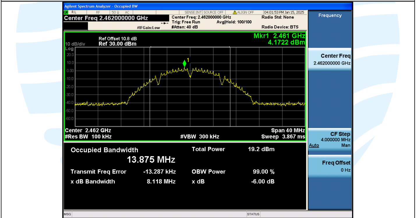
11B-Ant1-2462MHz-PASS
