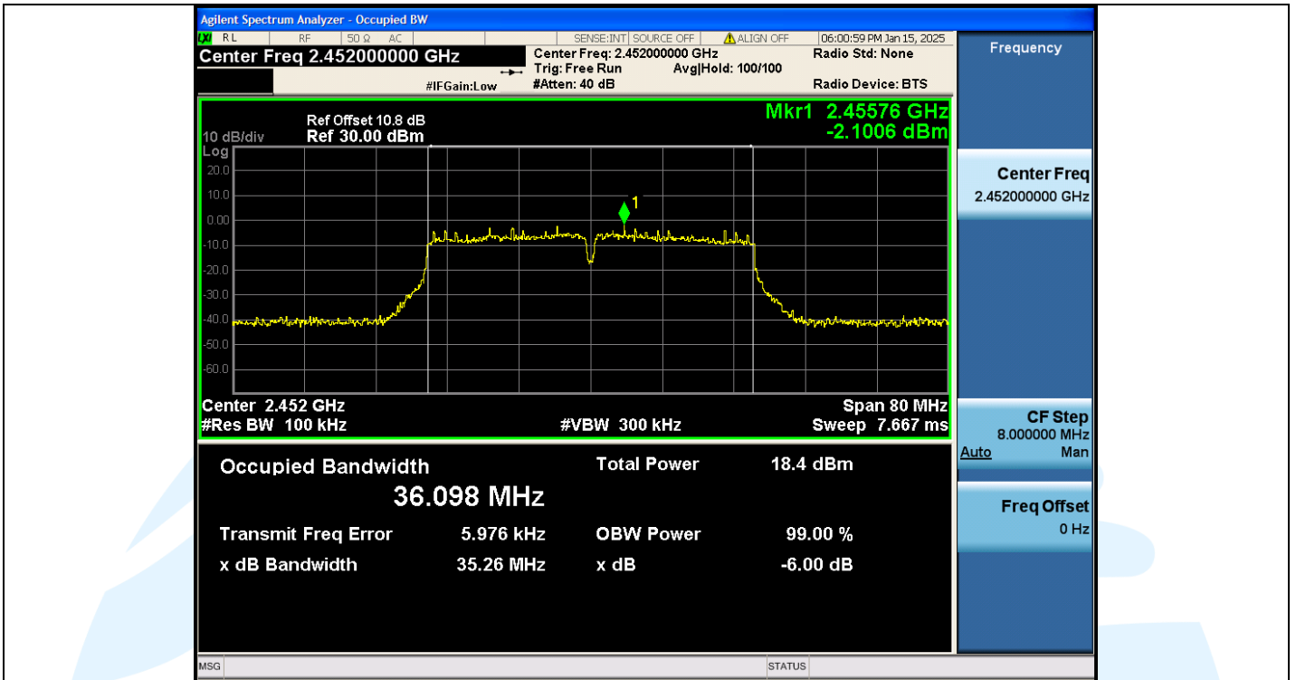
11N40SISO-Ant1-2452MHz-PASS
