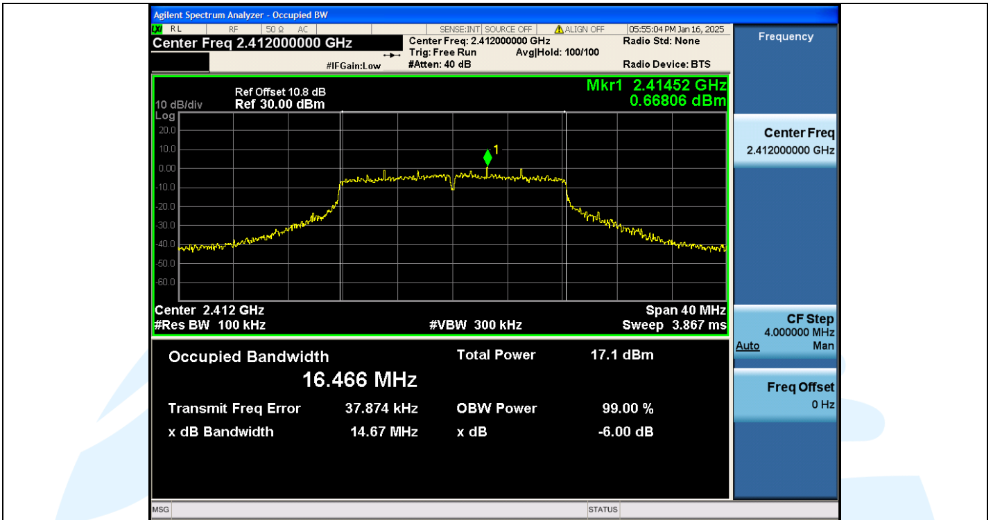
11G-Ant1-2412MHz-PASS
