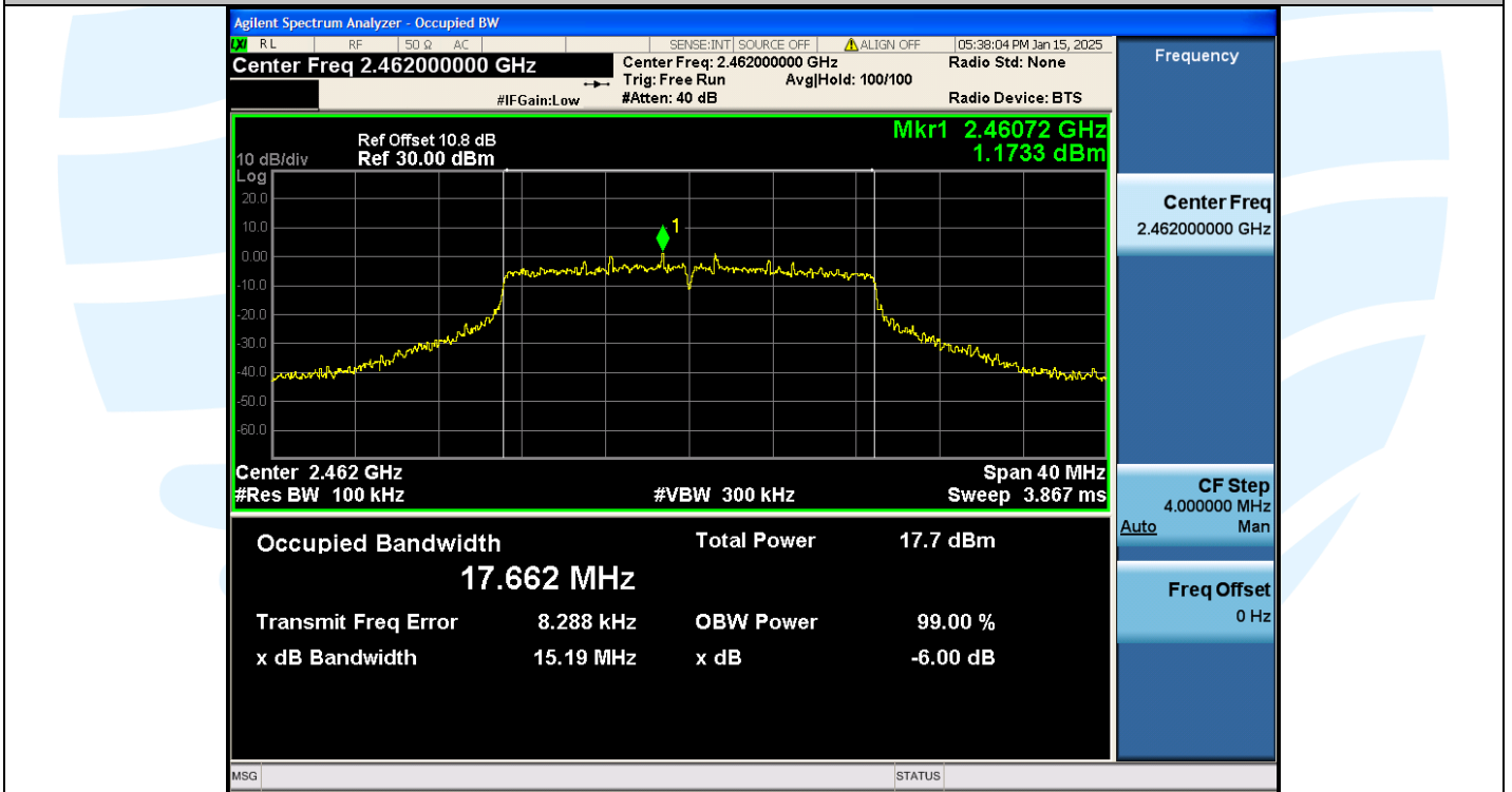
11N20SISO-Ant1-2462MHz-PASS
