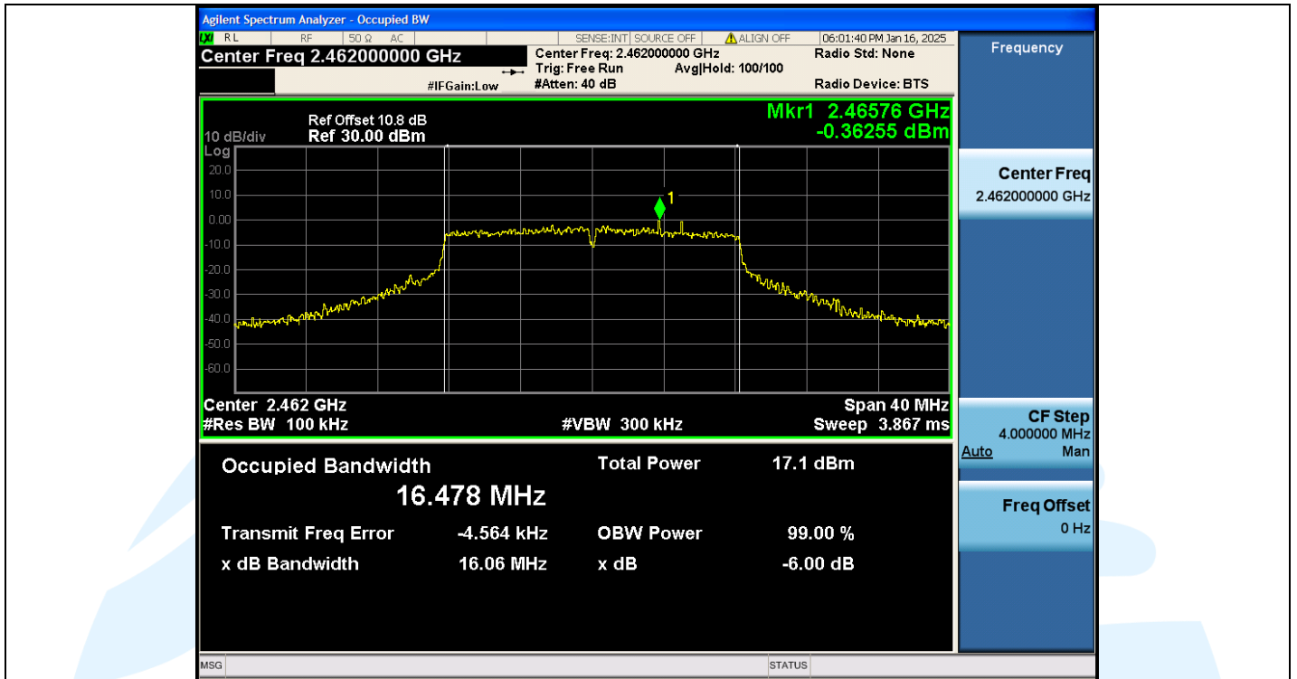
11G-Ant1-2462MHz-PASS
