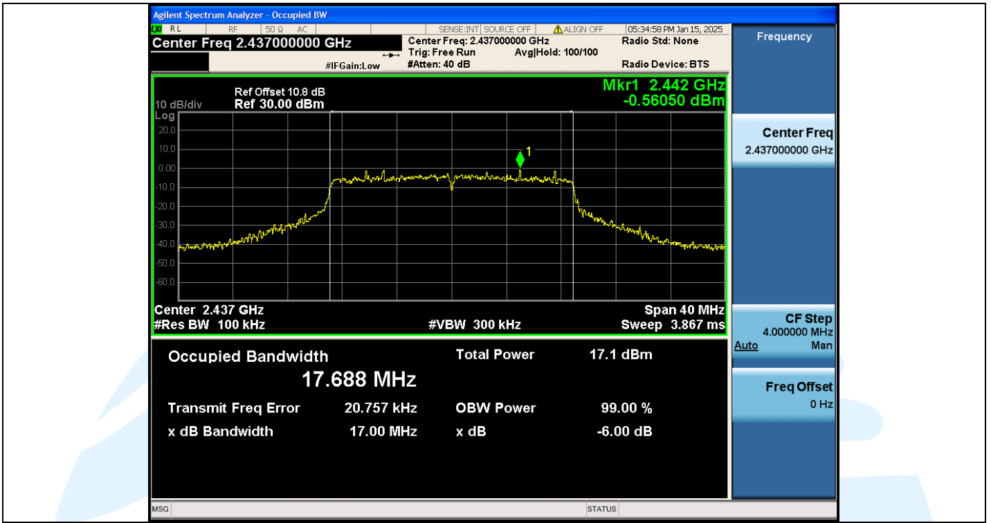
11N20SISO-Ant1-2437MHz-PASS
