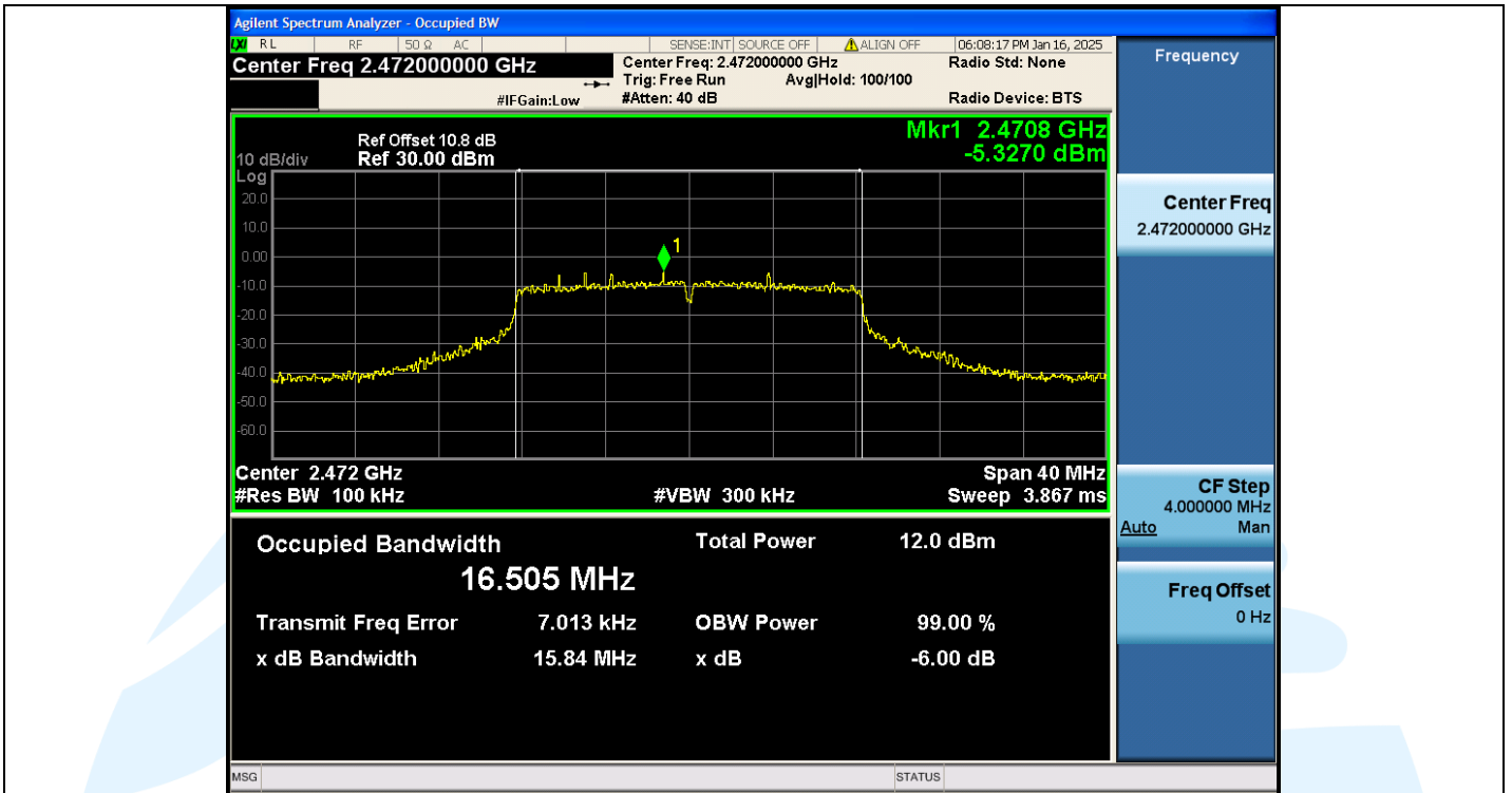
11G-Ant1-2472MHz-PASS
