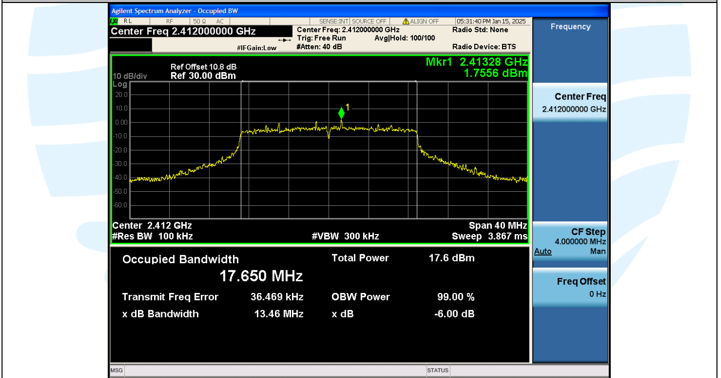
11N20SISO-Ant1-2412MHz-PASS
