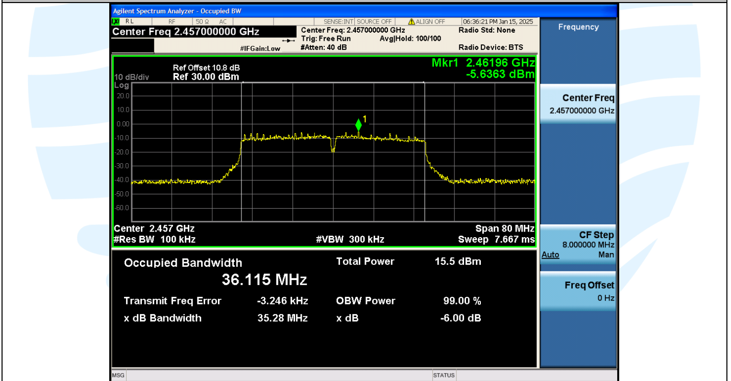
11N40SISO-Ant1-2457MHz-PASS
