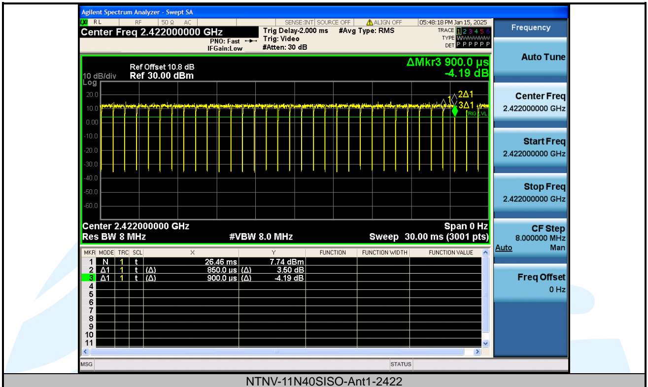
NTNV-11N40SISO-Ant1-2422
