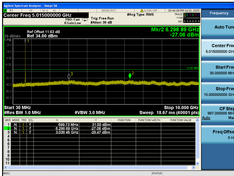
LTE Band 12 / 10 MHz / 16QAM - RB Size/Offset (1/0) – Low Channel
