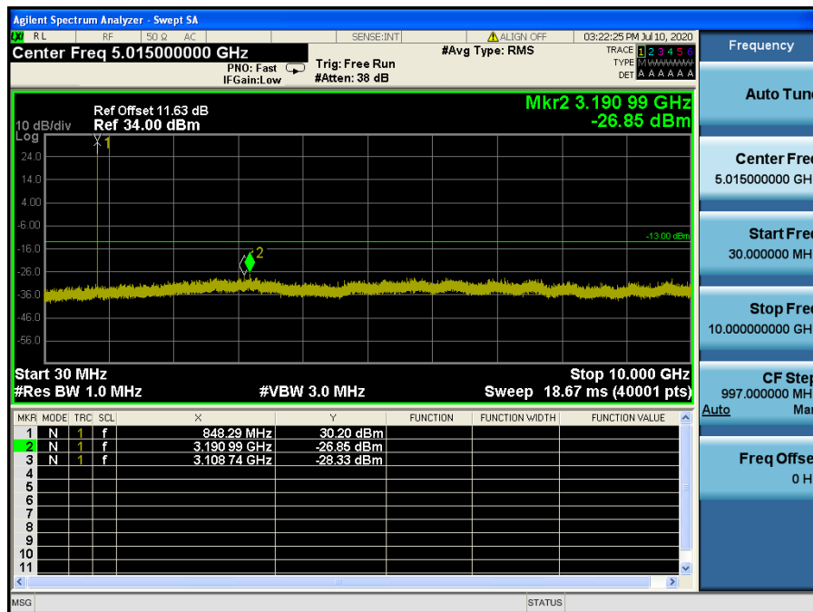
LTE Band 5 / 1.4 MHz / 16QAM - RB Size/Offset (3/0) – High Channel
