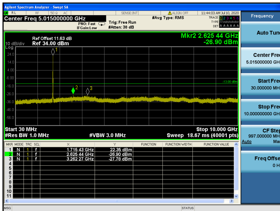
LTE Band 4 / 20 MHz / 16QAM - RB Size/Offset (50/0) – Low Channel
