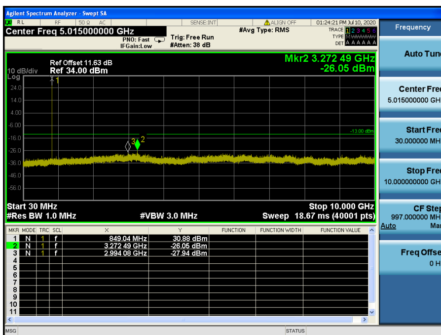
LTE Band 5 / 3MHz / QPSK - RB Size/Offset (1/14) – High Channel
