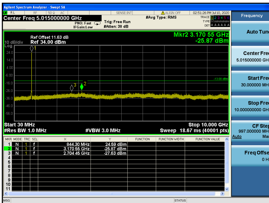
LTE Band 5 / 10 MHz / QPSK - RB Size/Offset (50/0) – High Channel
