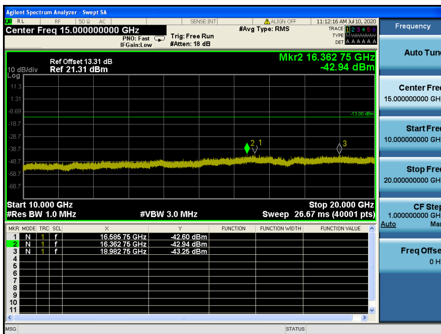
LTE Band 4 / 15 MHz / 16QAM - RB Size/Offset (36/0) – Mid Channel
