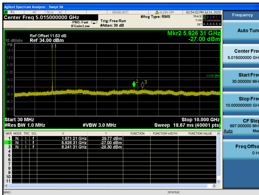
LTE Band 2 / 20 MHz / QPSK - RB Size/Offset (1/0) – Mid Channel
