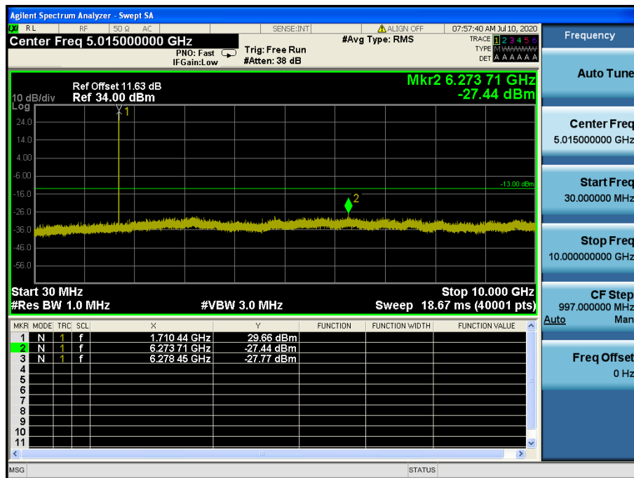
LTE Band 4 / 1.4 MHz / 16QAM - RB Size/Offset (1/0) – Low Channel
