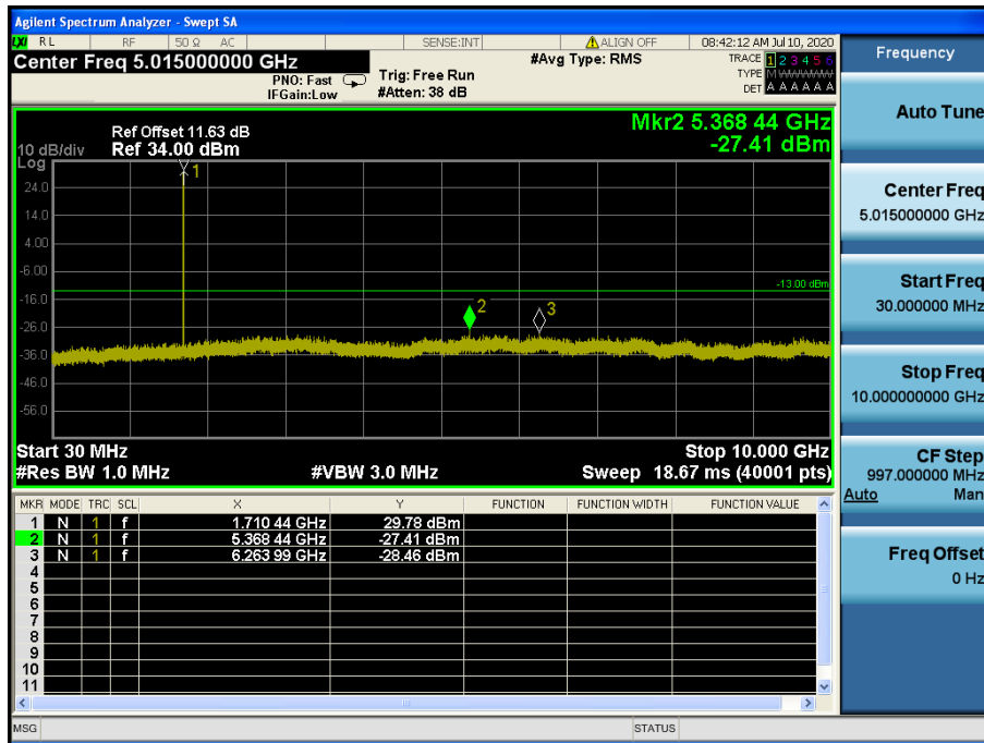
LTE Band 4 / 3MHz / 16QAM - RB Size/Offset (1/0) – Low Channel
