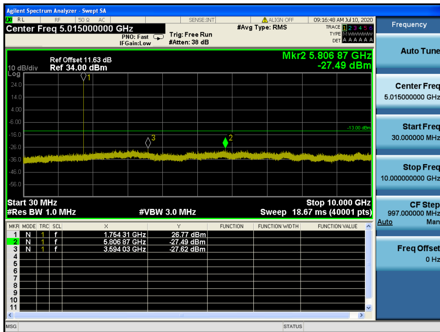
LTE Band 4 / 3MHz / 16QAM - RB Size/Offset (8/4) – High Channel
