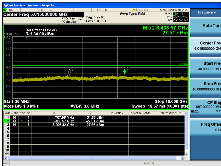
LTE Band 12 / 1.4 MHz / QPSK - RB Size/Offset (3/3) – Mid Channel
