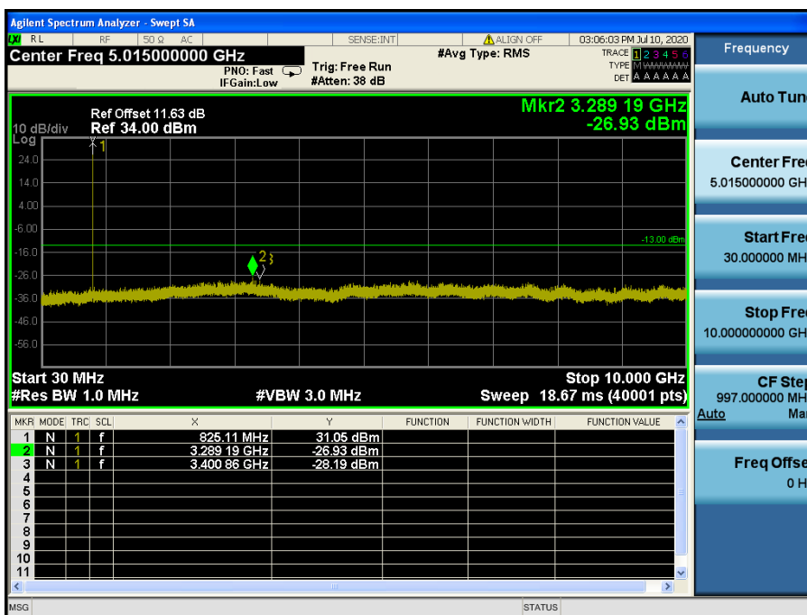
LTE Band 5 / 1.4 MHz / 16QAM - RB Size/Offset (3/3) – Low Channel
