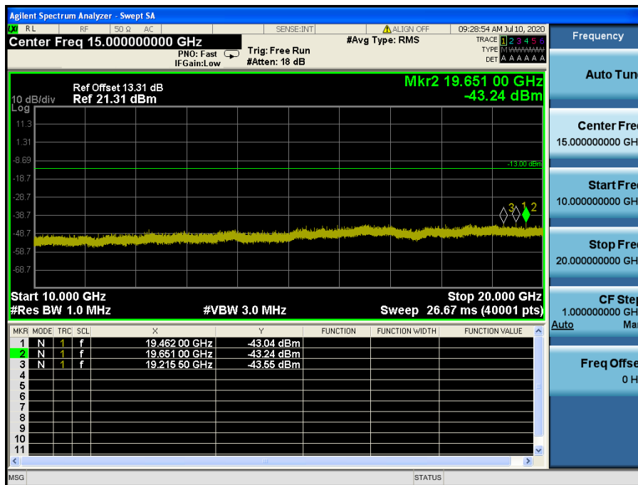
LTE Band 4 / 5 MHz / 16QAM - RB Size/Offset (1/12) – Low Channel
