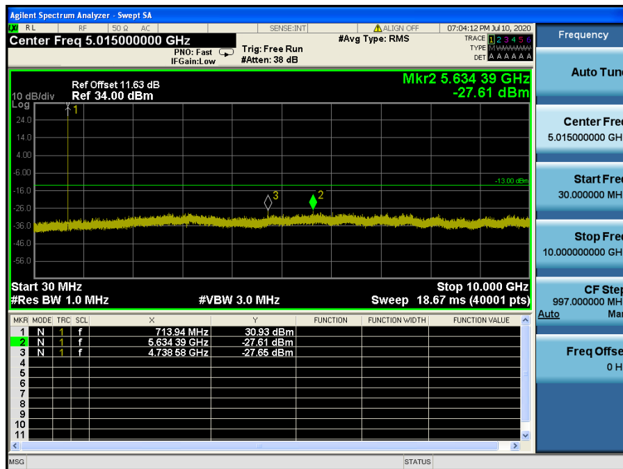
LTE Band 12 / 5 MHz / QPSK - RB Size/Offset (1/12) – High Channel
