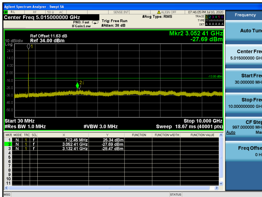
LTE Band 12 / 10 MHz / QPSK- RB Size/Offset (25/25) – High Channel
