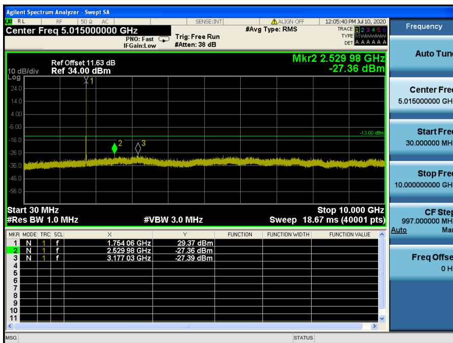
LTE Band 4 / 20 MHz / 16QAM - RB Size/Offset (1/99) – High Channel
