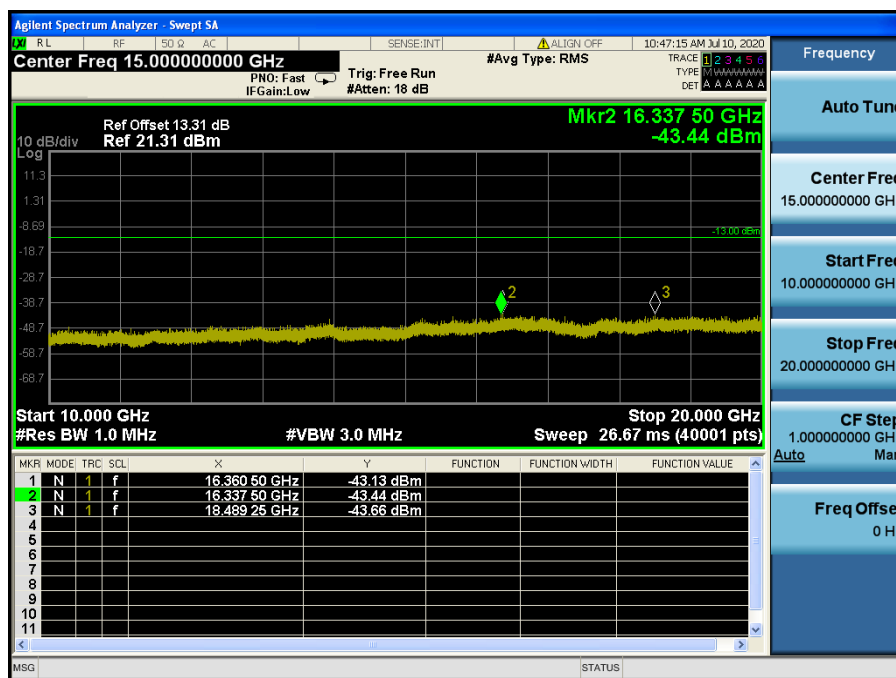
LTE Band 4 / 10 MHz / 16QAM - RB Size/Offset (25/25) – High Channel
