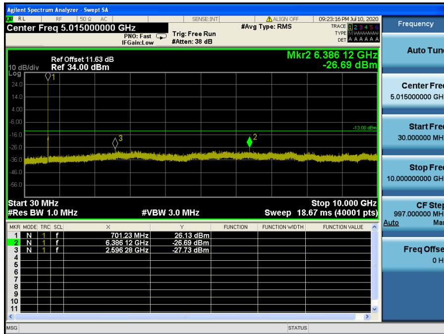
LTE Band 12 / 5 MHz / 16QAM - RB Size/Offset (25/0) – Low Channel
