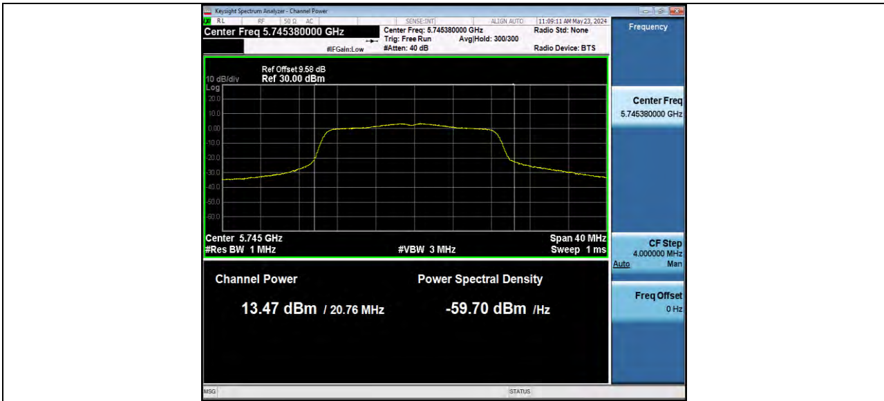
11AC20MIMO Ant2 5745
