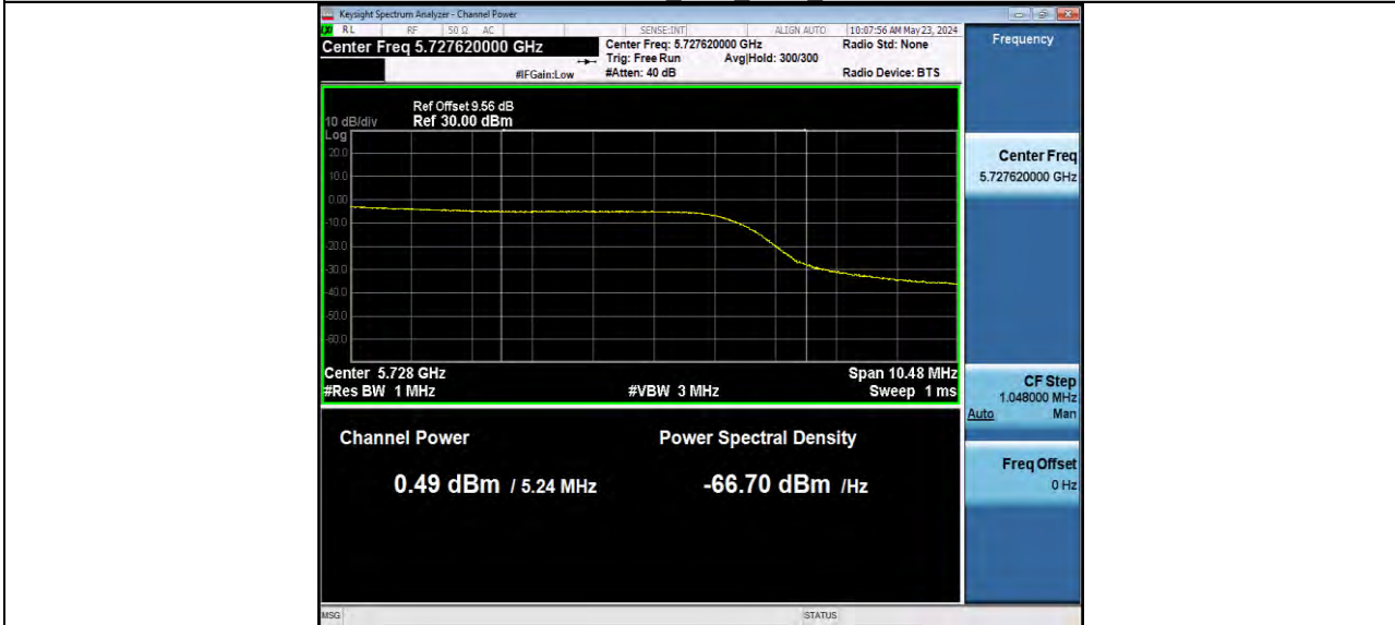
11AC20MIMO Ant1 5745
