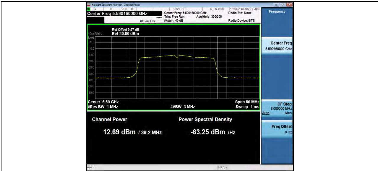
11N40MIMO Ant2 5590
