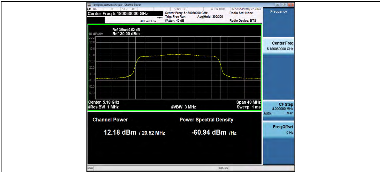
11AX20MIMO Ant2 5180
