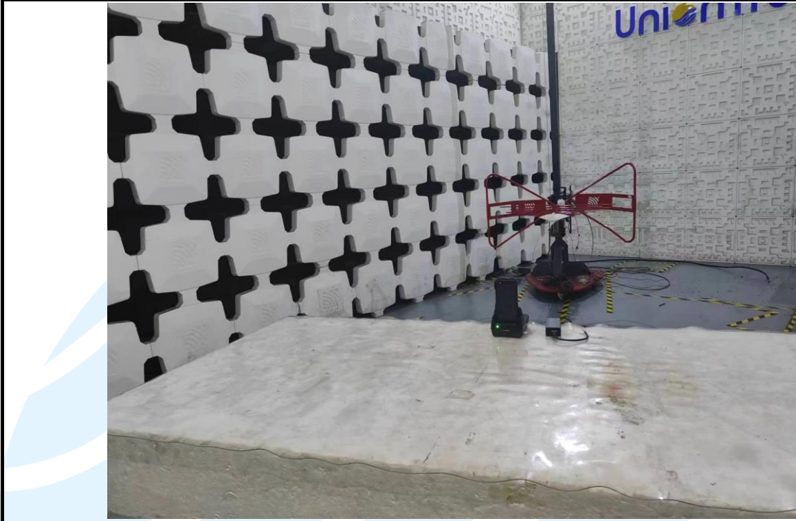
Radiated emission Test Setup-1 (30 MHz~1 GHz) _Test Mode 7
