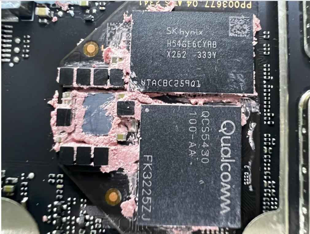
Internal View of EUT-69
