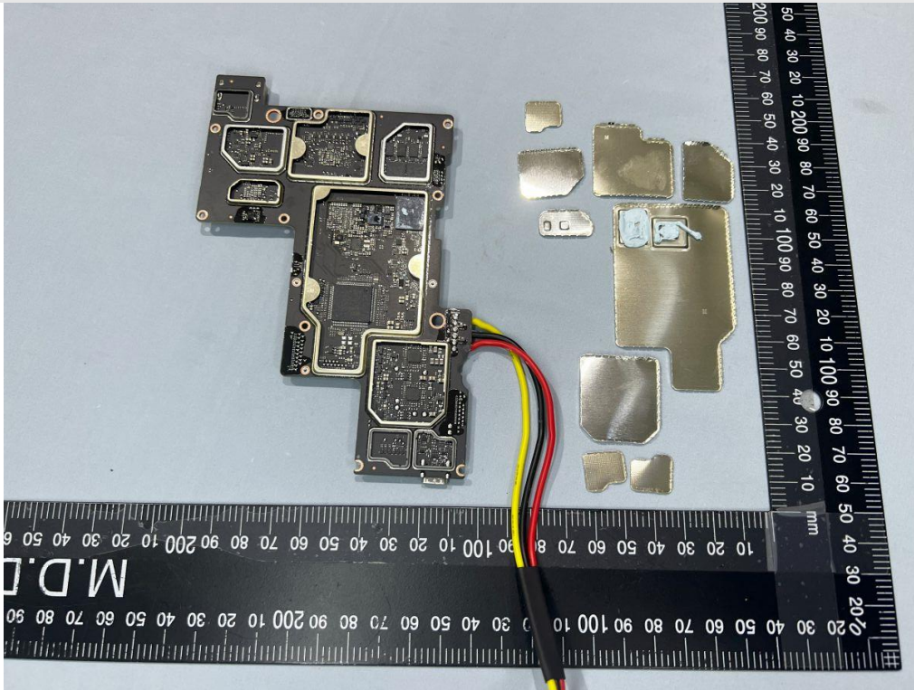
Internal View of EUT-75
