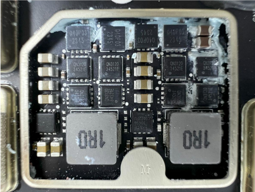
Internal View of EUT-73
