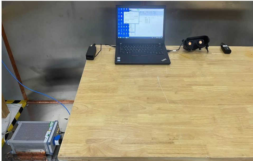
Photograph 3: Set-up photo for Conducted Emission on AC Mains
