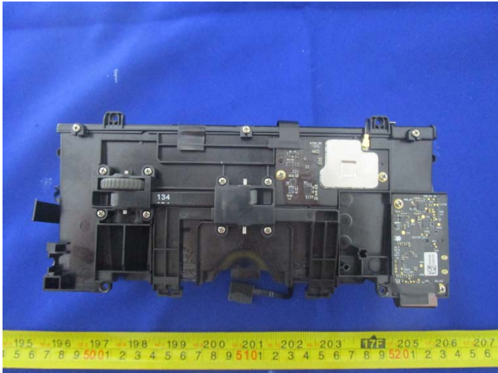
EUT – Main Part Bottom View
