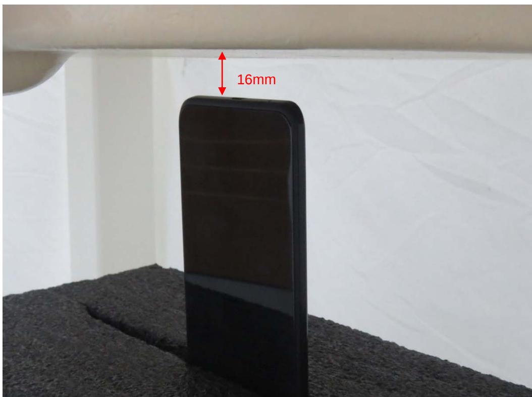
Picture 6: Bottom Edge, the distance from handset to the bottom of the Phantom is 16mm
