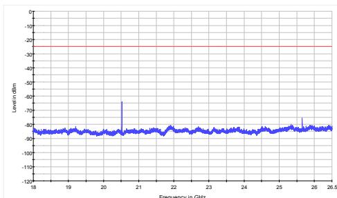
LTE Band 7 5MHz CH-High 18GHz~26.5GHz
