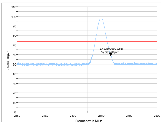
DH5-Channel 78: Peak
