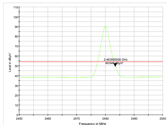
DH5-Channel 78: Average
