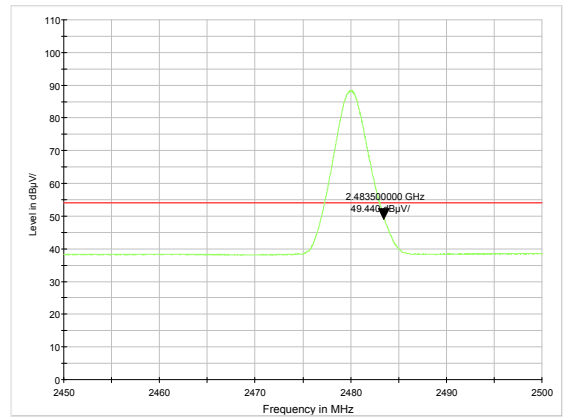
3DH5-Channel 78: Average
