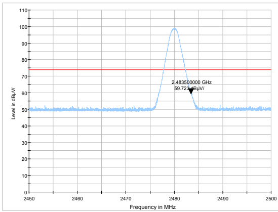
3DH5-Channel 78: Peak
