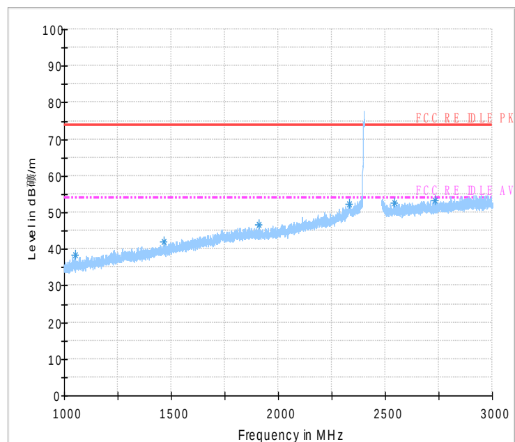
Fig.47 Radiated Spurious Emission (802.11b,Ch1,1GHz~3GHz)
