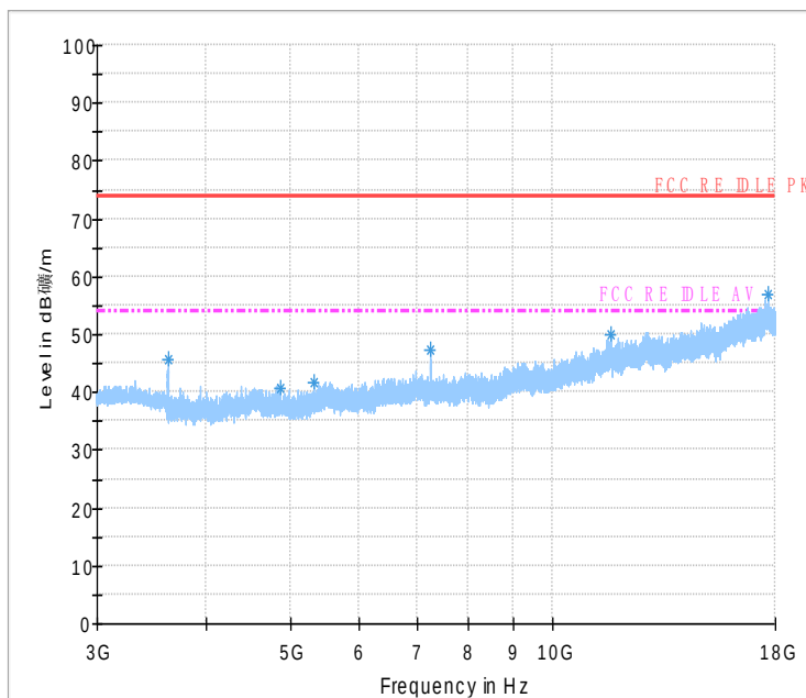
Fig.48 Radiated Spurious Emission (802.11b,Ch1,3GHz~18GHz)
