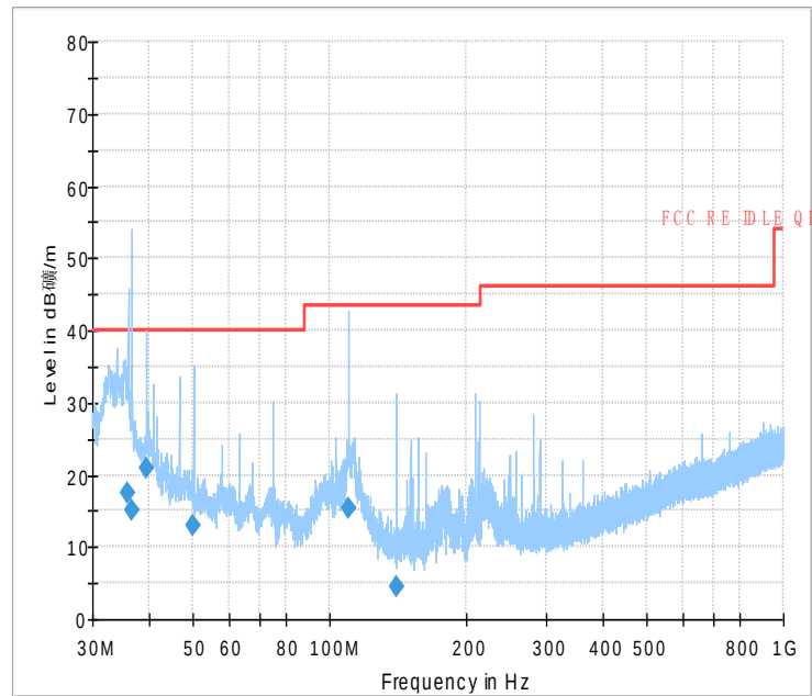
Fig.46 Radiated Spurious Emission (802.11b,Ch1,30MHz~1GHz)
