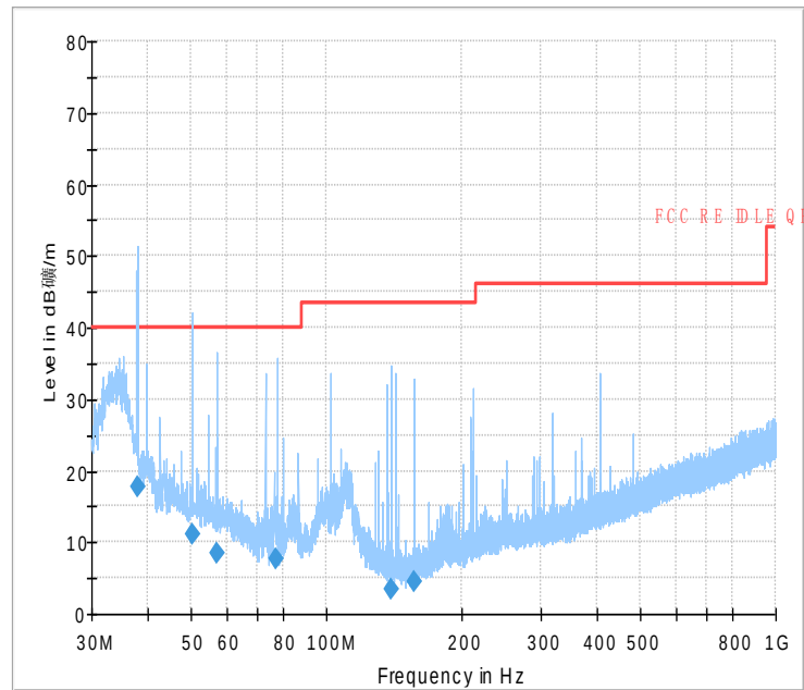
Fig.56 Radiated Spurious Emission (802.11 n-20MHz,Ch1,30MHz~1GHz)
