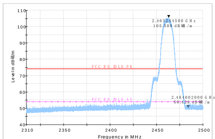
Fig.45 Radiated emission (Power): 802.11b, high channel
