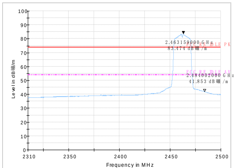
Fig.50 Radiated emission (Power): 802.11g, high channel
