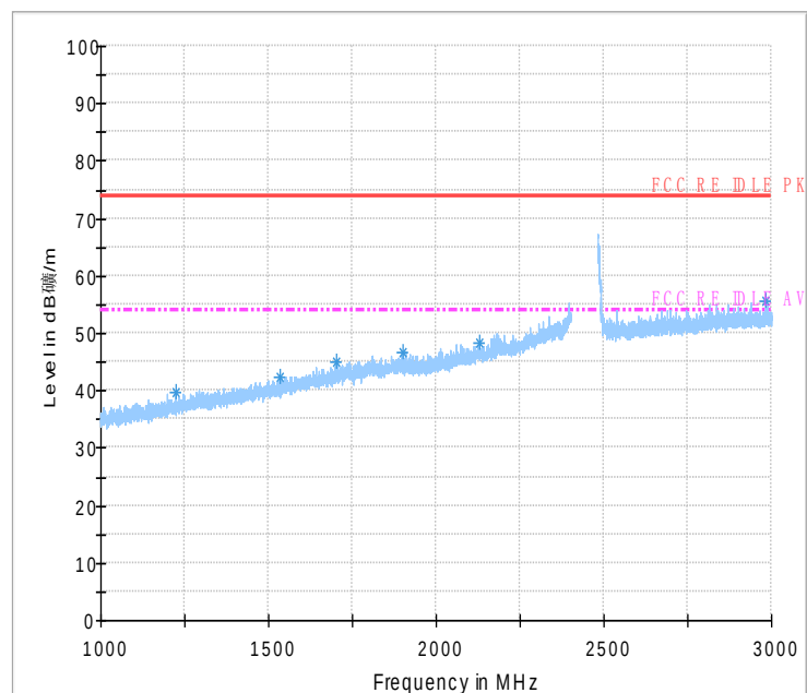
Fig.57 Radiated Spurious Emission (802.11 n-20MHz,Ch1,1GHz~3GHz)
