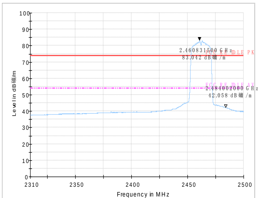
Fig.55 Radiated emission (Power): 802.11n, high channel
