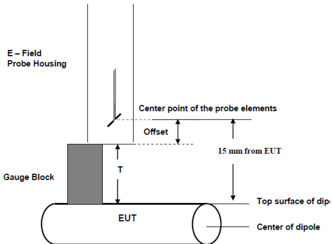
Fig. 9.2 Gauge block with E-field probe
