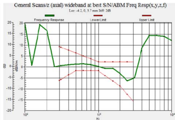
Fig 7.2 GSM1900 Ch661
