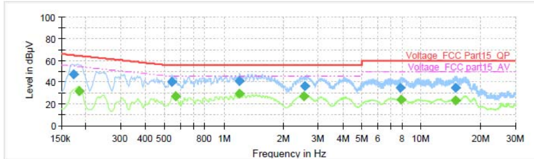
WIFI_L_0.15-30MHz
