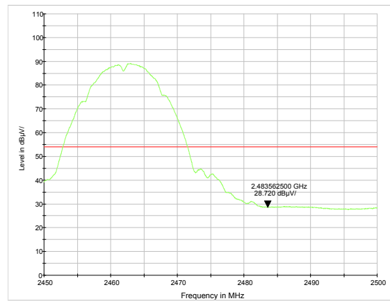
802.11g-Channel 11: Peak
